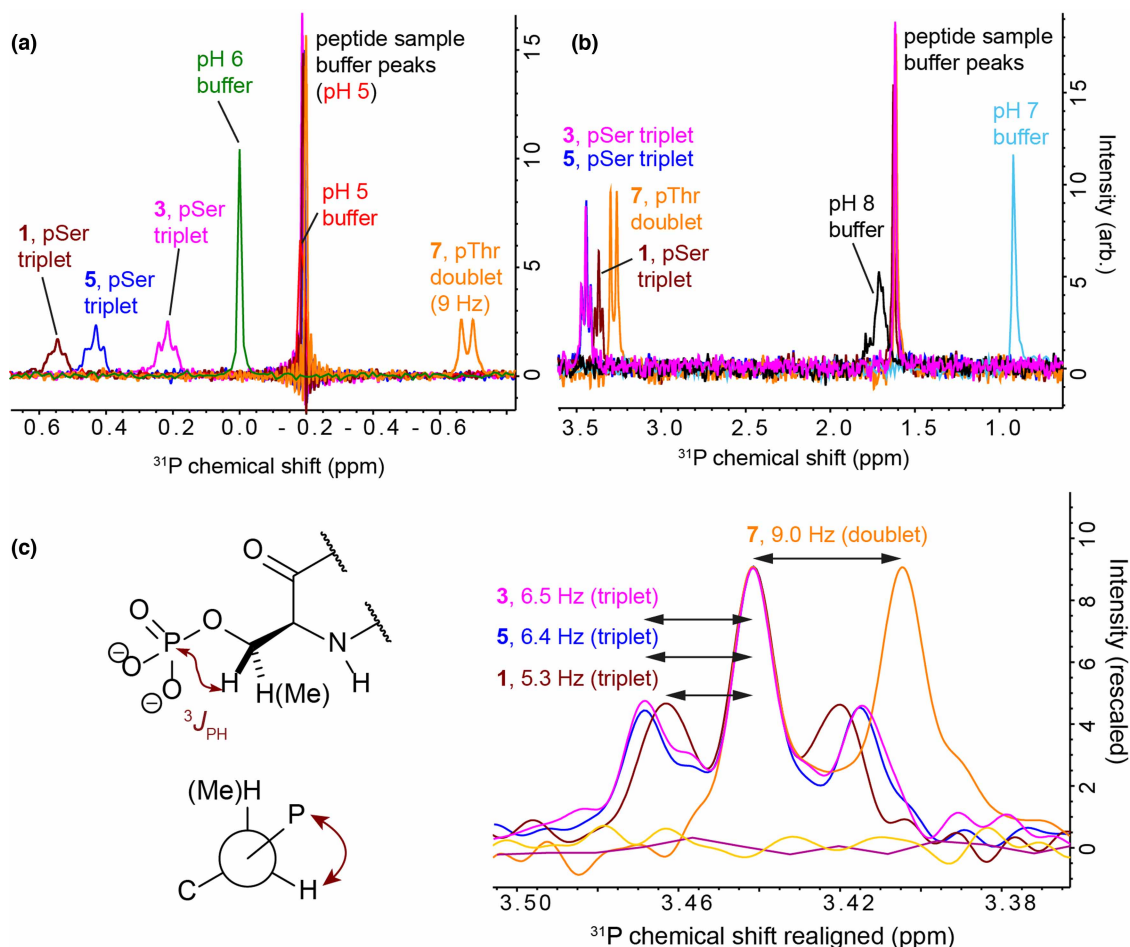
Figure 7. ^{31}\text{P} NMR spectra for selected peptides (1, 3, 5, 6 and 7) and CD buffer standards at pH 5, 6, 7 and 8.
