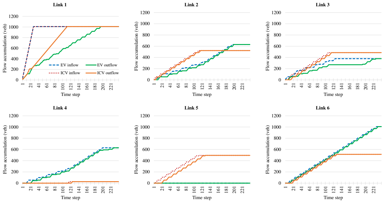
Figure 3: Inflow-outflow profiles of each vehicle class
