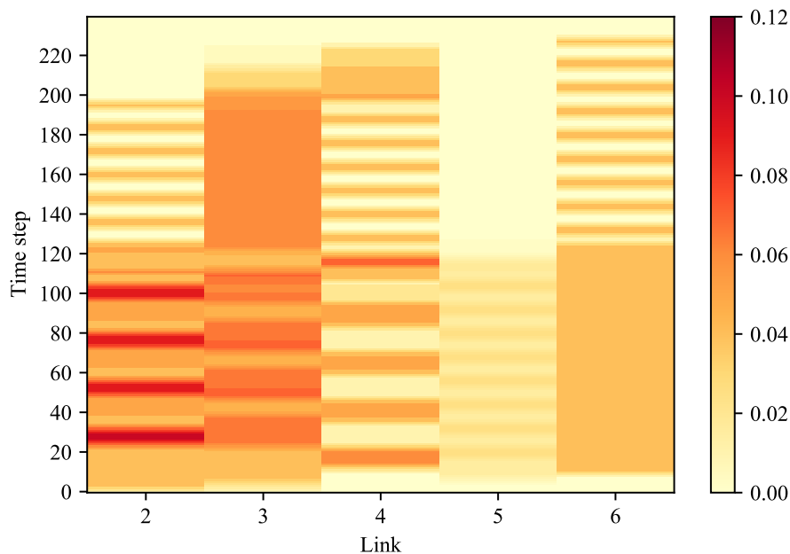
Figure 5: The density on each link over the time horizon (veh/m)
