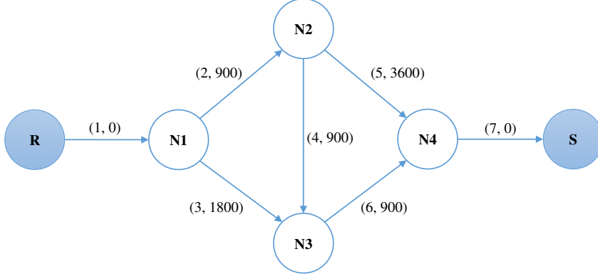
Figure 2: Braess network
