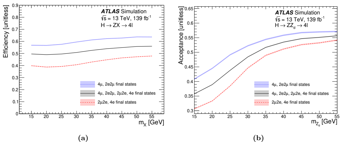
Figure 15. (a) Model-independent efficiencies \epsilon_c for the H \rightarrow ZX process for different combinations of the final states calculated in the fiducial volumes described in table 6. (b) Model-dependent per-channel fiducial region acceptances for the H \rightarrow ZZ_d \rightarrow 4\ell process for different combinations of the final states.
