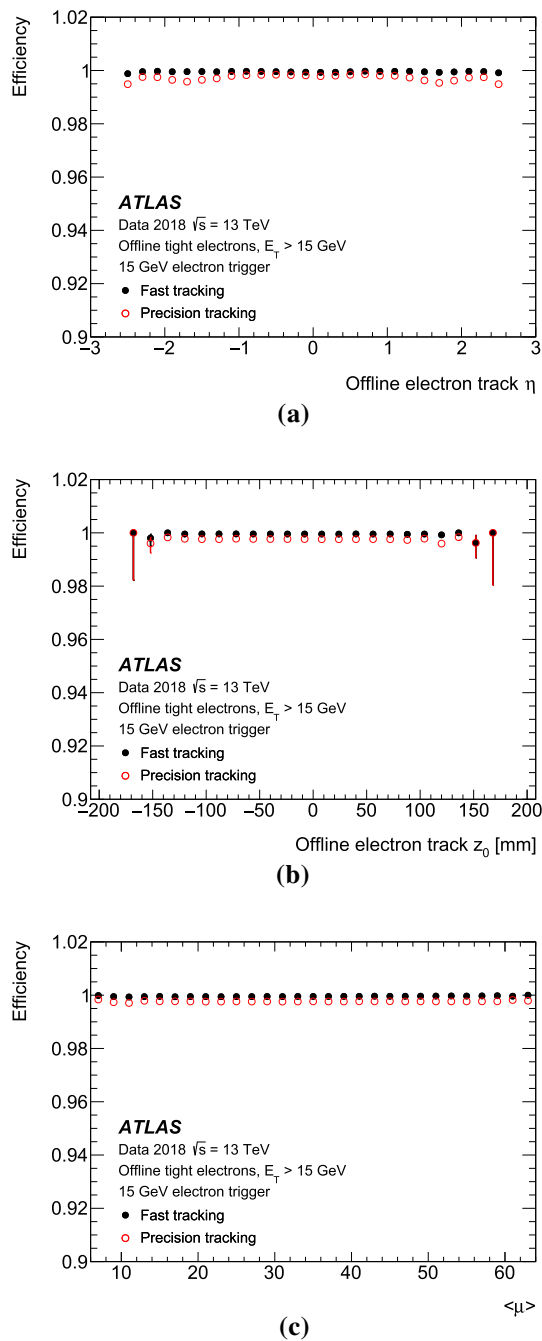
Fig. 28 The electron track finding efficiency versus a the offline electron track pseudorapidity, b z_0 position at the beam line, and c the mean pile-up interaction multiplicity measured using the dilepton trigger
