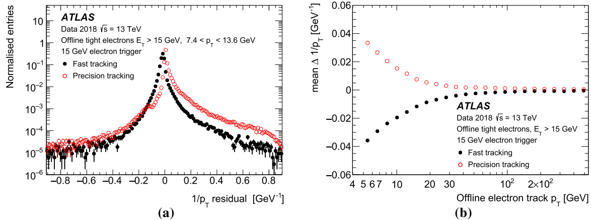
Fig. 31 The ID trigger residual in 1/p_T with respect to offline for the fast and precision tracking for electron candidates with the offline track transverse momentum the range in 7.4 < p_T < 13.6 \text{ GeV} selected by
