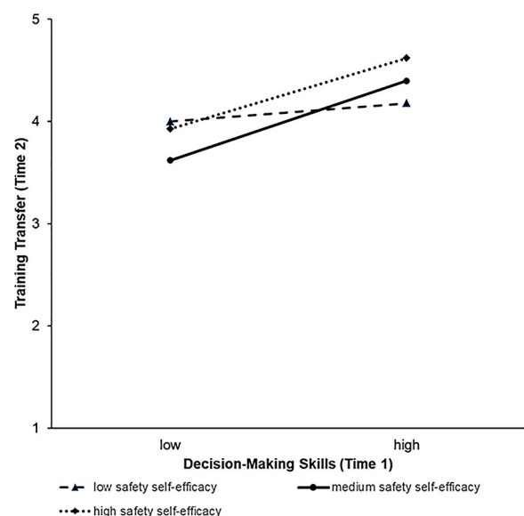
Figure 2. Form of interaction between decision-making skills (T1) and safety self-efficacy (T1) on training transfer (T2).
