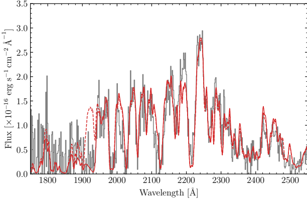
Figure 2. NUV spectrum of SDSS J0956+5912 (grey). The best fitting model and a similar model with carbon removed are shown by the red solid/dashed curves, respectively.
