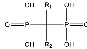
FIGURE 1 | The generic structure of a bisphosphonate. This figure was created by using ChemDraw software.
