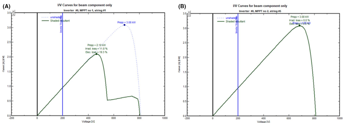
FIGURE 6 Impact of the shading calculation on the power curve at 12.45 PM. (A) Sub-array 1 string 1 in which is the string that has the highest degree of shading. (B) Sub-array 1 strings 5 (both Huawei inverter)
