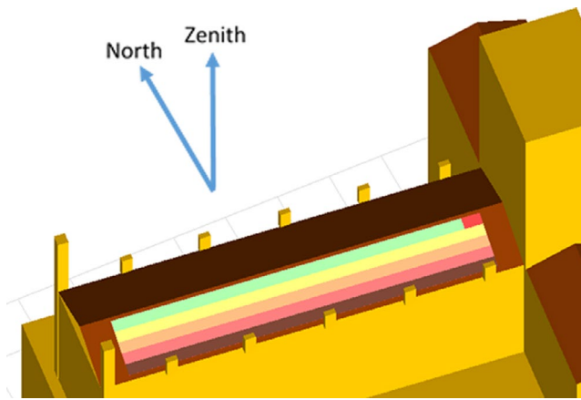
FIGURE 7 Module strings layout showing the exposure of strings 1–2 to shading from the crenellations
