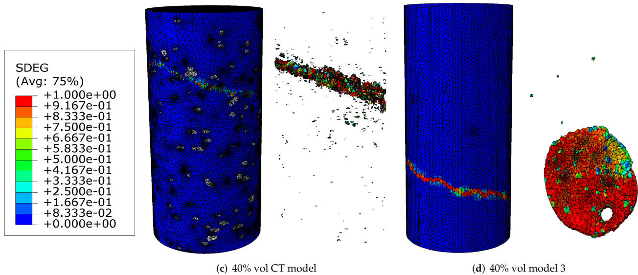
Figure 11. (a) Stress-strain curves, (b) energy output and (c,d) crack patterns of 40% vol parametric and CT concrete models under tension [31].
