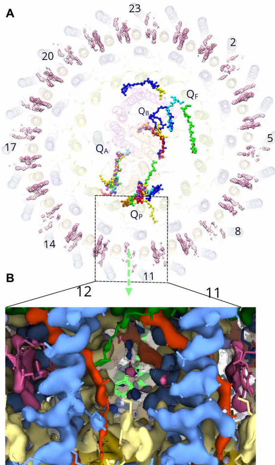
Fig. 5. The Q P quinol export site in the RC-dLH complex. (A) The RC-dLH complex viewed from the cytoplasmic side of the membrane, with all details partly obscured, and showing the densities for B800 BChls (pink) in the outer LHh ring. Structurally resolved quinones for the G. phototrophica complex are shown (green), with those for the RC-LH1 complexes from Rhodospseudomonas palustris W-minus (16) (blue), R. palustris W-plus (16) (cyan), T. tepidum (11) (yellow), Thiorhodovibrio stain 970 (17) (purple), and Blastochloris viridis (9) (red). The green arrow indicates a likely path for quinol export, at a position of weak B800 density. The positions of LHh subunit are numbered. (B) Two LHh \alpha/\beta units 11 and 12 viewed in the plane of the membrane showing the proposed position for quinol export that corresponds to a low or zero occupancy B800 site; LHh- \alpha (pale yellow), LHh- \beta (cornflower blue), gemmatoxanthin (orange red), B800 (pink), B816 (dark green), and Q P (bright green). The cryo-EM map is shown at two contour levels (opaque surface = 7.0 \sigma ; wireframe = 7.5 \sigma ).
