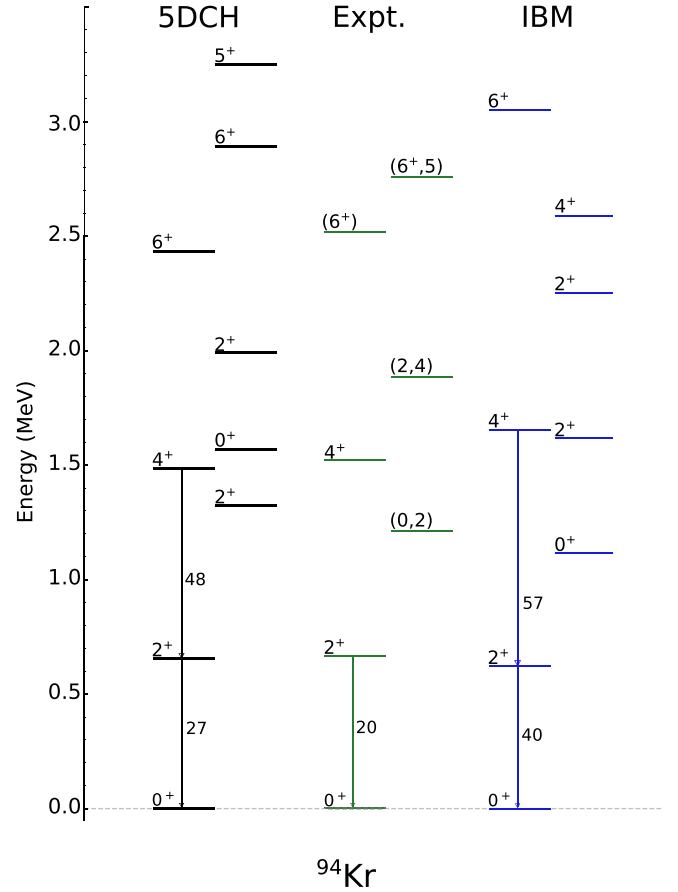
FIG. 12. Theoretical low-energy excitation levels of ^{94}\text{Kr} compared with experimental values [14,33]. Levels in black (left) were calculated using a 5DCH, in blue (right) using the mapped IBM [18]. E2 transition strengths in W.u. are shown along the arrows. See text for more details.
