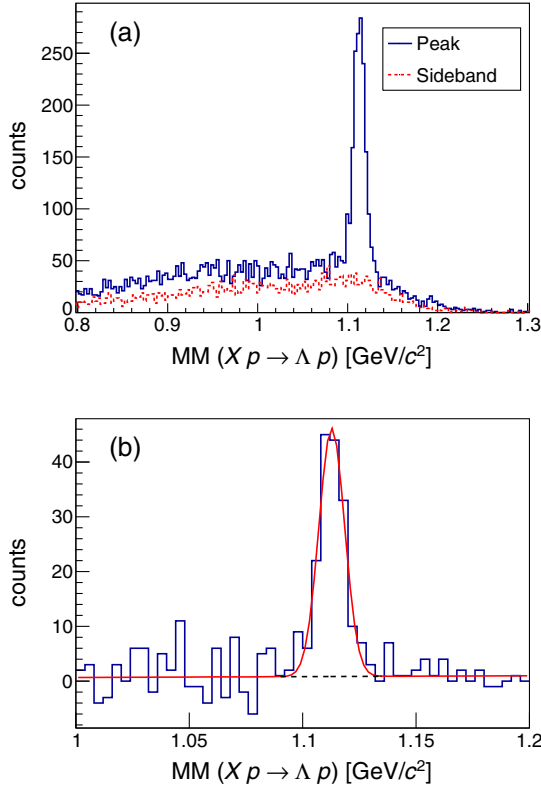
FIG. 4. Missing mass distribution of the secondary vertex integrated over all momentum ranges (top) and binned in the incident \Lambda momentum range 1.3–1.4 GeV/ c after sideband subtraction (bottom). The solid line in (a) represents the data selected in the peak region of Fig. 2(a), while the dotted line represents the sideband region. The solid line in (b) shows the total fit including the peak, which is fit to a Gaussian function. The dashed line represents the background, which is fit to a constant.
