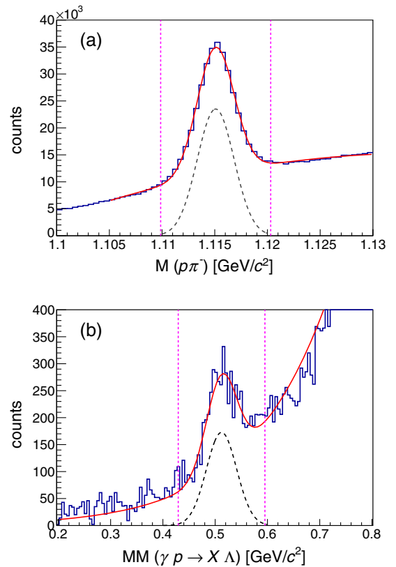
FIG. 2. Mass spectrum of the detected proton and \pi^- (top) from the decayed \Lambda' and the missing mass spectrum of the initial vertex (bottom). The missing mass spectrum (bottom) was plotted after the cut was made around the \Lambda' mass (top). The total fit, peak plus background, is shown by the solid line. The Gaussian fits, shown by the dashed lines, are for reference only, and are not used in the cross section calculation. The vertical lines frame the data that pass through to the final analysis.
