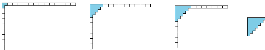
FIGURE 3. Some examples of framed staircases: \alpha = \tau_{(1^8)}^{(13)}, \tau_{(1^6)}^{(9)}, \tau_{(1^5)}^{(7)} , and \tau = \rho(9) are all partitions of n = 45 . Up to conjugation, there are 35 framed staircase partitions of n = 45 . The classification of decomposable Specht modules labelled by framed staircases is the main result of [DG18]. In Theorem 5.5 we prove Saxl's conjecture for all framed staircase partitions. The key ingredient in our proof is that (\tau_{(1^b)}^{(a)}, \tau_{\emptyset}^{(a+b)}) is a 1-Carter-Saxl pair for a, b \in \mathbb{N} .
