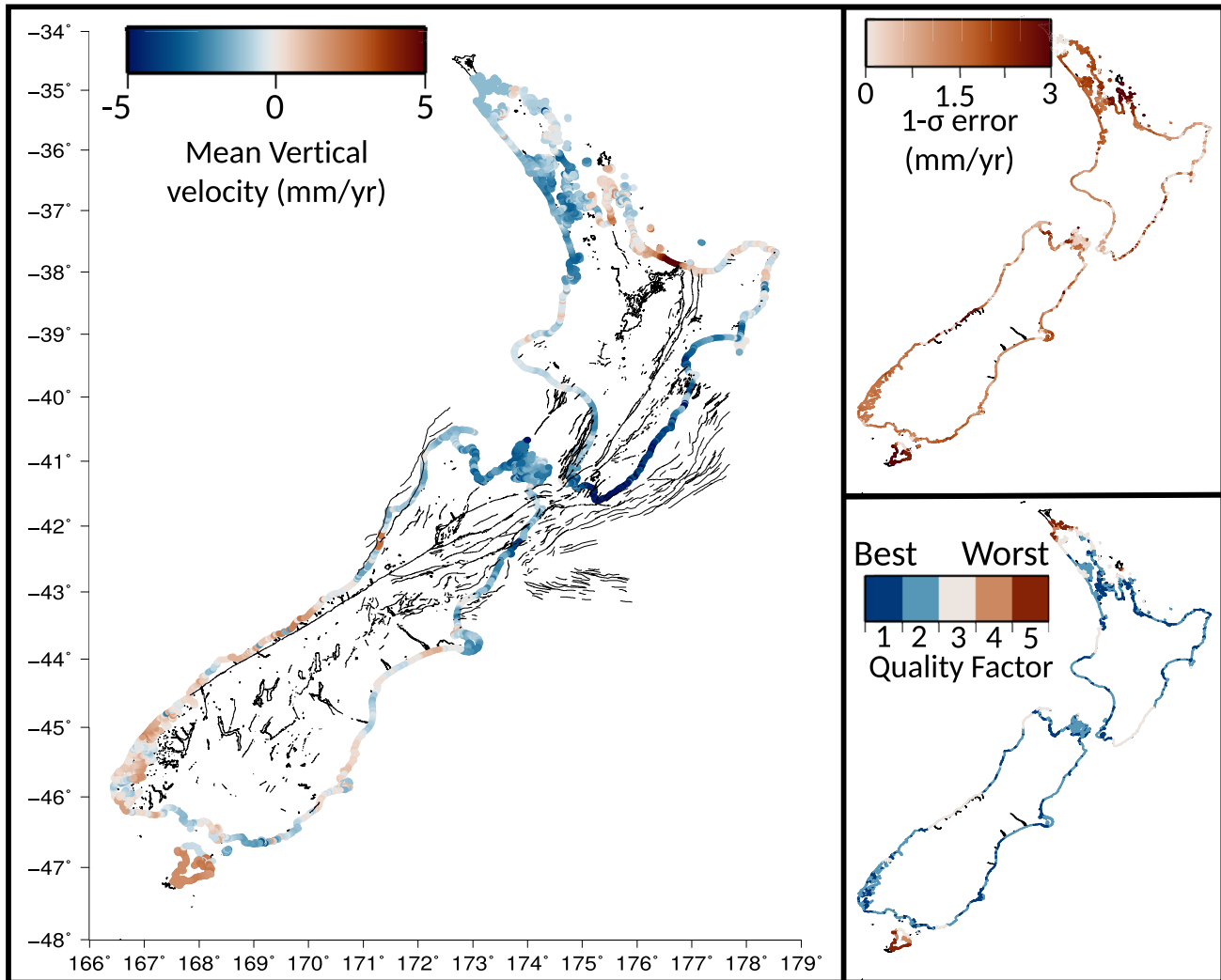
Figure 4. The main figure shows the VLM for the New Zealand coastline. The two panels on the right show the 1- \sigma uncertainties and the quality factor (Table S1 in Supporting Information S1).
