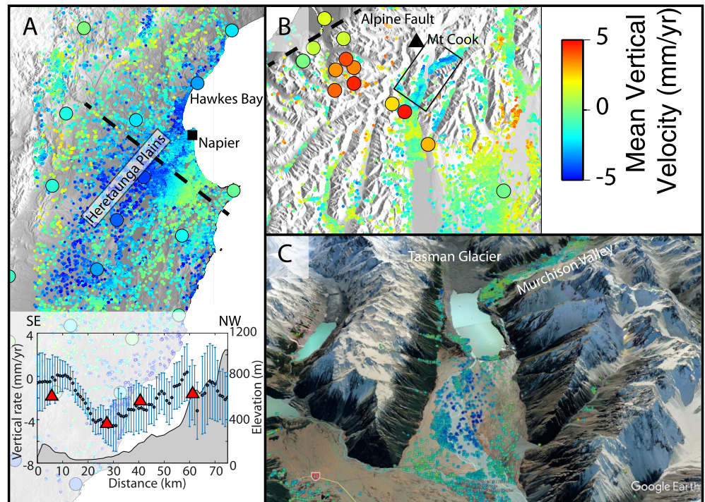
Figure 3. (a) Zoom-in of the vertical deformation across Hawkes Bay and the Heretaunga Plains and profile showing the sharp transition to subsidence. (b) Zoom-in of the central Southern Alps highlighting the non-tectonic deformation along some of the glacial river valleys. The black triangle shows the location of Aoraki/Mt Cook (170.177 E, -43.585S). The black dashed line shows the location of the Alpine Fault, the black box shows the region covered in (c) and the colored circles are the GNSS derived vertical rates.
