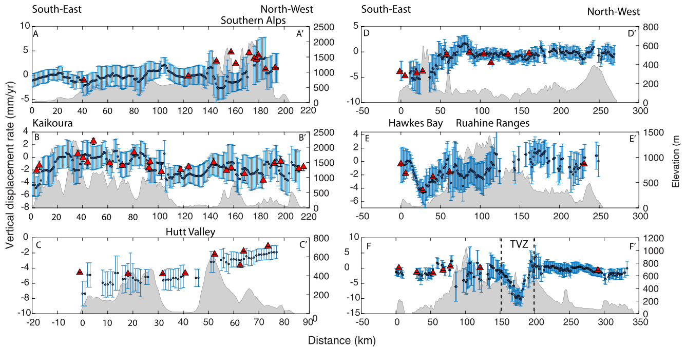
Figure 2. Profiles along six profiles shown in Figure 1. Blue dots and associated error bars are from the InSAR derived vertical velocities and the red dots are from GNSS located within 10 km of the profile. The gray polygons show the topography along each of the profiles. Locations, including Kaikōura, the Southern Alps and the TVZ are also highlighted.
