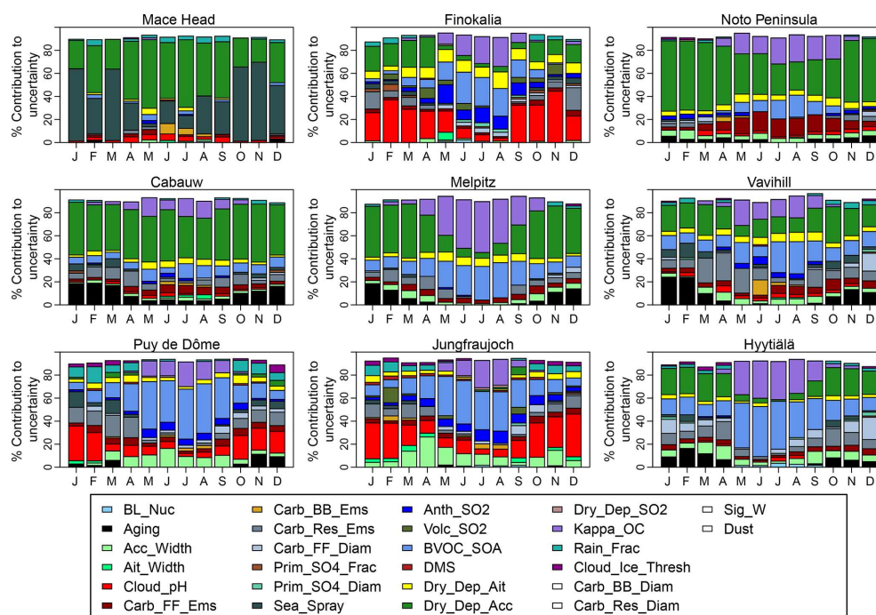
Figure 11. Contribution to the uncertainty in monthly average CCN_{0.2} based on HadGEM3-UKCA perturbed parameter ensemble simulations for the year 2008. Each color refers to 1 of the 26 perturbed parameters as indicated in the legend of the figure. The uncertainty is shown as the percentage contribution of the parameter to the CCN_{0.2} variance. The assumed parameter uncertainty ranges are given in Yoshioka et al. (2019). All contributions smaller than 1% are not shown. Abbreviations are as follows. BL_Nuc: boundary layer nucleation; Aging: aging “rate” from insoluble to soluble; Acc_Width: modal width (accumulation soluble–insoluble); Ait_Width: modal width (Aitken soluble–insoluble); Cloud_pH: pH of cloud drops; Carb_FF_Ems: particle mass emission rate for BC and OC (fossil fuel); Carb_BB_Ems: particle mass emission rate for BC and OC (biomass burning); Carb_FF_Diam: particle emitted mode diameter for BC and OC (fossil fuel); Carb_BB_Diam: particle emitted mode diameter for BC and OC (biomass burning); Carb_Res_Diam: particle emitted mode diameter for BC and OC (biofuel); Prim_SO4_Frac: mass fraction of SO_2 converted to new SO_4^{-2} particles in sub-grid power plant plumes; Prim_SO4_Diam: mode diameter of new sub-grid SO_4^{-2} particles; Sea_Spray: sea spray mass flux (coarse / accumulation); Anth_SO2: SO_2 emission flux (anthropogenic); Volc_SO2: SO_2 emission flux (volcanic); BVOC_SOA: biogenic monoterpene production of SOA; DMS: DMS emission flux; Dry_Dep_Ait: dry deposition velocity of Aitken mode aerosol; Dry_Dep_Acc: dry deposition velocity of accumulation-mode aerosol; Dry_Dep_SO2: dry deposition velocity of SO_2 ; Kappa_OC: hygroscopicity parameter kappa for organic aerosols. Default value in UKCA is 0.06; see Petters and Kreidenweis (2007). Sig_W: standard deviation of updraft velocity (this affects the activation of aerosol particles to form cloud droplets). Dust: dust emission flux; Rain_Frac: the fraction of the cloudy part of the grid box in which rain is forming and hence scavenging takes place; Cloud_Ice_Thresh: scavenging (by both cloud liquid and ice water) is suppressed in dynamic clouds when cloud ice fraction is higher than this value. The parameters with no color in the legend do not contribute to the uncertainty in CCN_{0.2} (less than 1%) at any station in any month.
