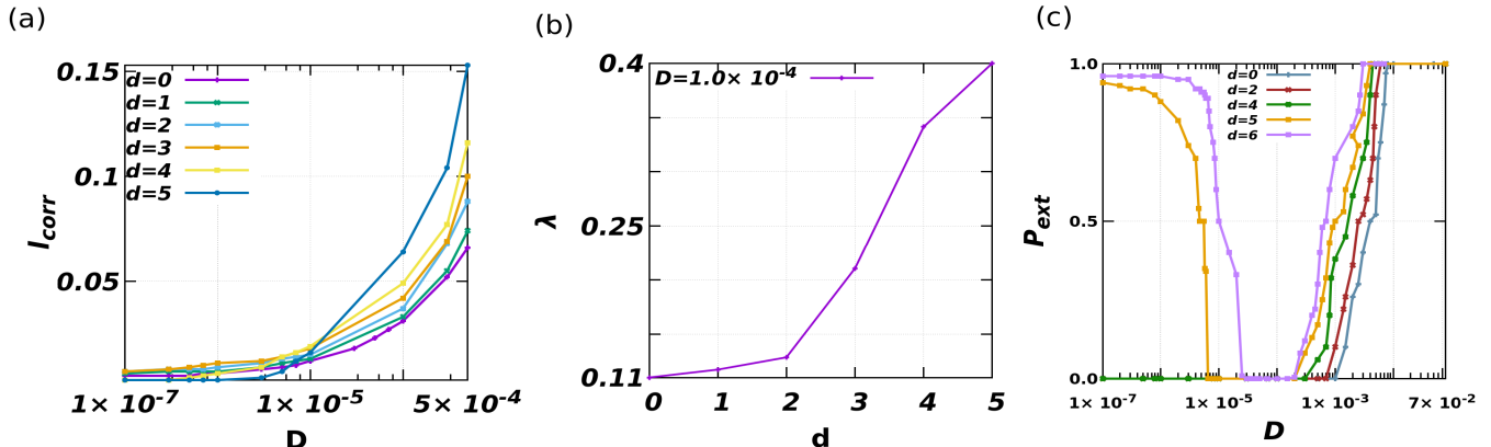
FIG. 4. (a) Correlation lengths ( l_{\text{corr}} ) are plotted against different mobility strengths ( D ). At higher diffusion, the length is enhanced. This is consistent with previous results [10]. If the death rate is increased, then the length is also sharply increased. In intermediate mobility strength ( D \sim 10^{-5} ), the species density “revives” (species coexistence) for higher death rate thus correlation becomes non zero (see the blue and yellow line). (b) The wavelength ( \lambda ) of the correlation function as a function of death ( d ) for a particular value of mobility ( D = 1.0 \times 10^{-4} ). The wavelength is increasing as we increase the death value. This indicates the spirals increase in size with increasing death rate. (c) Extinction probability as a function of mobility D . Five death rates have been chosen. For higher death rates ( d = 5, 6 ), the extinction probability is high for low ( D \sim 10^{-7} ) and high ( D \gtrsim 10^{-3} ) diffusion, and goes to zero in the intermediate values of D \sim 10^{-4} .
