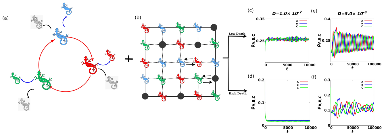
FIG. 1. Schematic diagram of cyclic interaction and mobility in presence of natural death. (a) Red arrows represent the cyclic predation between three species (red, blue, and green). Blue and black arrows reflect the reproduction and natural death respectively. (b) Mobility or exchange between two nearest neighbours (one of them may be vacant site). (c) and (e) At low death rate ( d = 1 ), the densities of species remain finite for two mobility strength : smaller D = 1 \times 10^{-7} as well as in higher value D = 5 \times 10^{-4} . (d) At high death rate ( d = 4 ) and for low diffusion, the density of each species is almost zero and no oscillatory behaviour is observed there. However (f) in the presence of higher diffusion, the oscillation with higher amplitude appears. In all the cases, 1000 \times 1000 lattice has been considered with unnormalized predation and reproduction rates, p = 7 and r = 7 respectively for each of the species.
