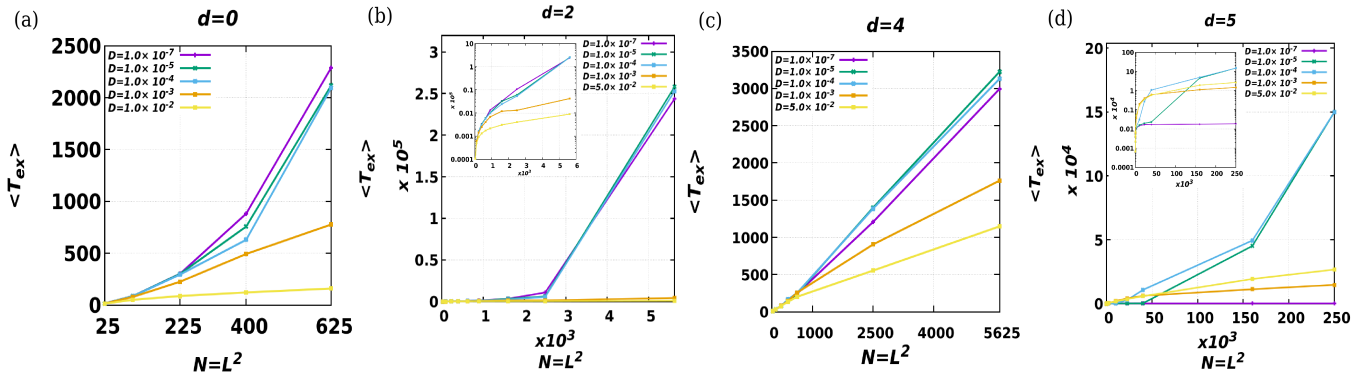
FIG. 5. Effect of lattice size on average extinction time at different death rates and mobility parameters: \langle T_{\text{ex}} \rangle is plotted against lattice size, N ( = L^2 ) for different death rates ( d ) and mobility ( D ). (a-b) Diffusion dominates for low death rates as it lowers the extinction time. (c-d) For high death rates both low and high diffusivity show lower extinction times whereas \langle T_{\text{ex}} \rangle is raised for an intermediate range of diffusion. Note that in (d) data for d = 5 , N = 500^2 and D = 10^{-4} and D = 10^{-5} are given as eye guides since coexistence is not lost at time 1.5 \times 10^5 (hence, in these cases \langle T_{\text{ex}} \rangle > 1.5 \times 10^5 ), see text. Insets of (b) and (d): \langle T_{\text{ex}} \rangle vs. N on lin-log scale. In this work, in one time step there are N elementary update moves corresponding to N = L^2 Monte Carlo steps.
