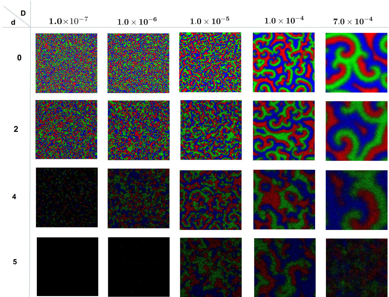
FIG. 3. Spatial plot of species density for different death rate and mobility strength. Distribution of the species throughout the lattice is shown by colours : Red, Green and Blue for A , B , and C respectively. Black dots are used for blank space. Diffusion strength is increased from 10^{-7} to 7 \times 10^{-4} (from left to right). Natural death rate is increased from zero to 5 (upper to bottom).
