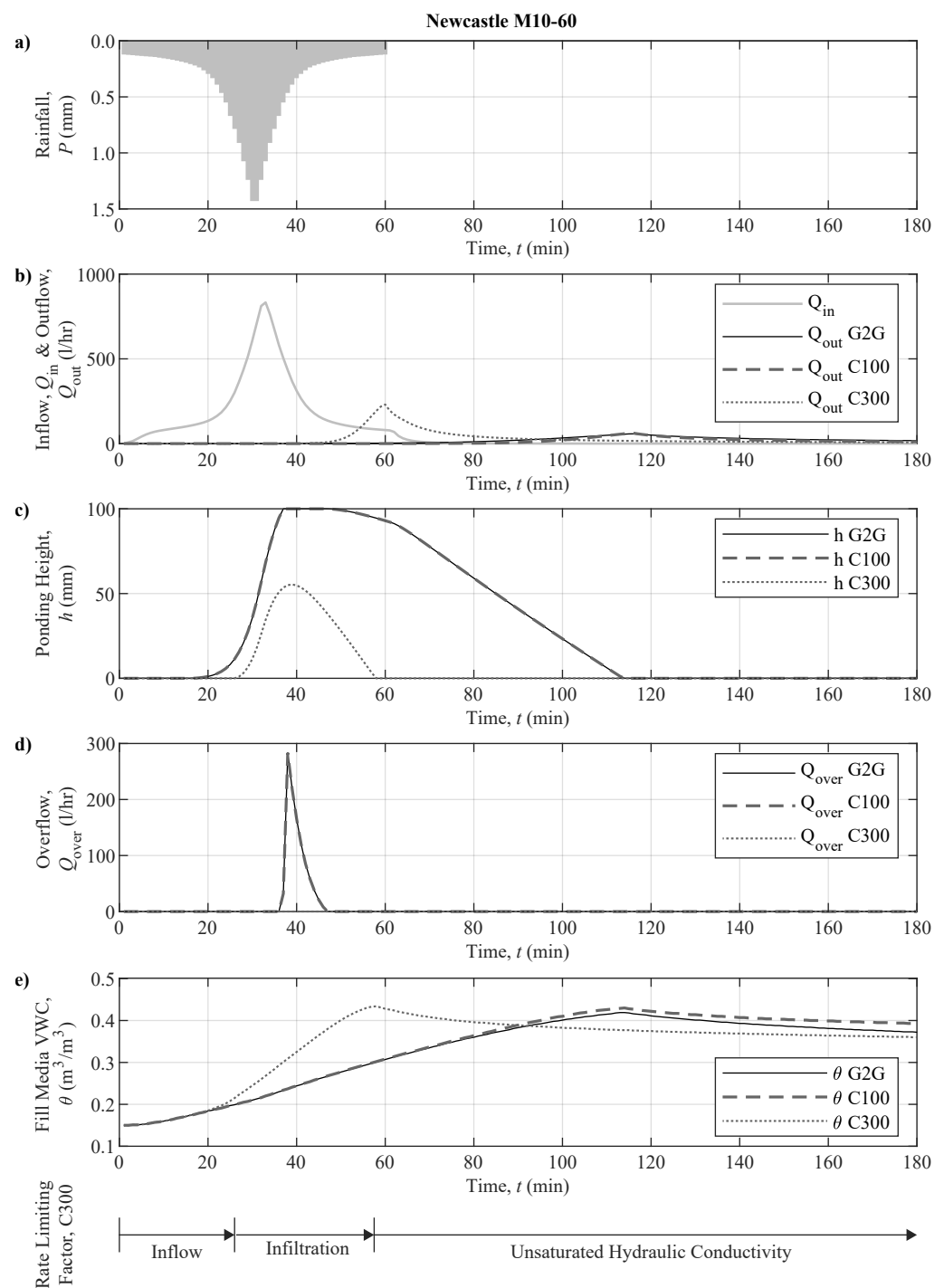
Figure 6. Modelled hydraulic response of bioretention systems in response to a 10-year return period 60-min duration storm event for Newcastle, UK. (a) Rainfall depth; (b) system inflow and outflow; (c) ponding height; (d) overflow; and (e) volumetric water content (VWC) of the fill media.
