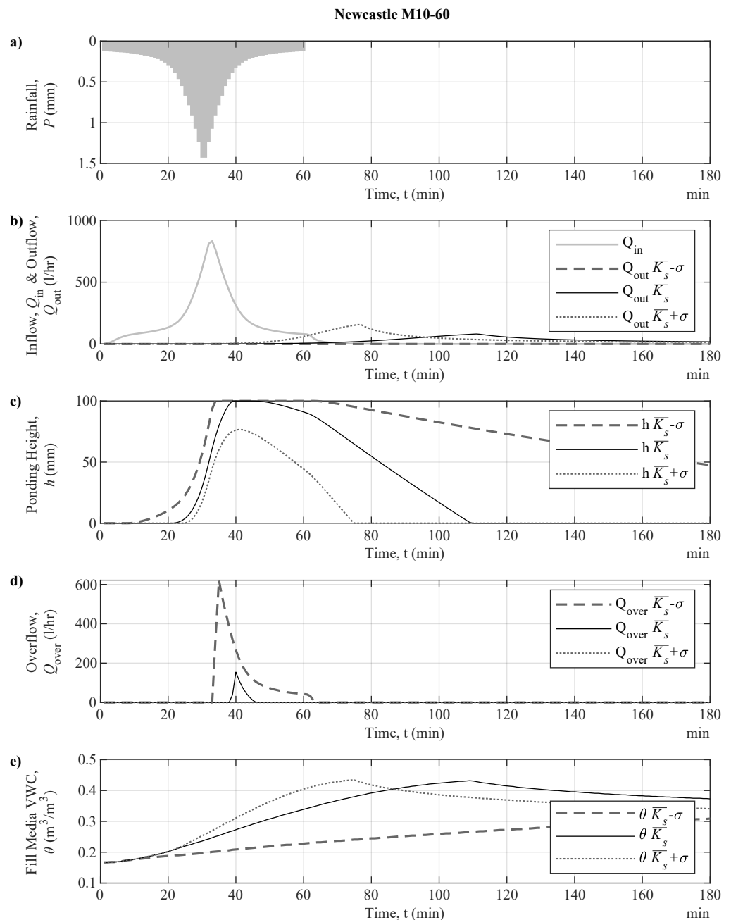
Figure 7. Modelled hydraulic response of the G2G bioretention system with mean saturated hydraulic conductivity ( \bar{K}_s ), mean saturated hydraulic conductivity minus 1 standard deviation ( \bar{K}_s - \sigma ) and mean saturated hydraulic conductivity plus 1 standard deviation ( \bar{K}_s + \sigma ) in response to a 10-year return period 60-min duration storm event for Newcastle, UK. (a) Rainfall depth; (b) system inflow and outflow; (c) ponding height; (d) overflow; and (e) volumetric water content (VWC) of the fill media.
