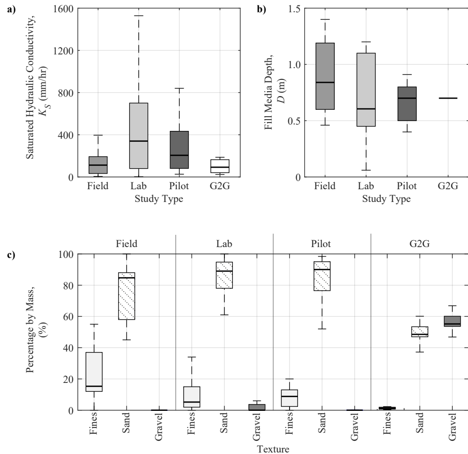
Figure 4. Comparison of G2G and literature examples of fill media physical characteristics: (a) saturated hydraulic conductivity; (b) media depth; and (c) media texture, fines (<0.063 mm), sand (0.063–2.0 mm) and gravel (>2.0 mm).
