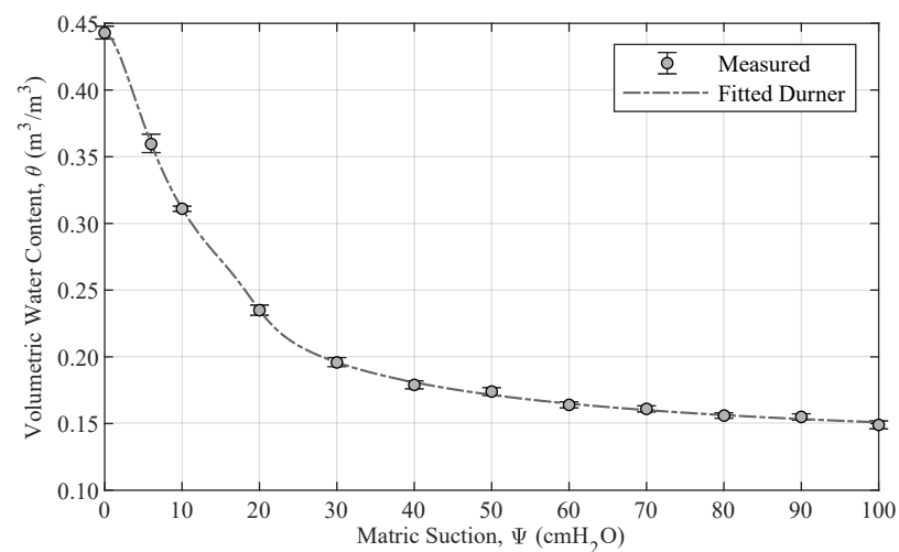
Figure 2. Measured Soil Water Release Curve for the G2G media and fitted Durner model. Error bars represent \pm 1 standard deviation.
