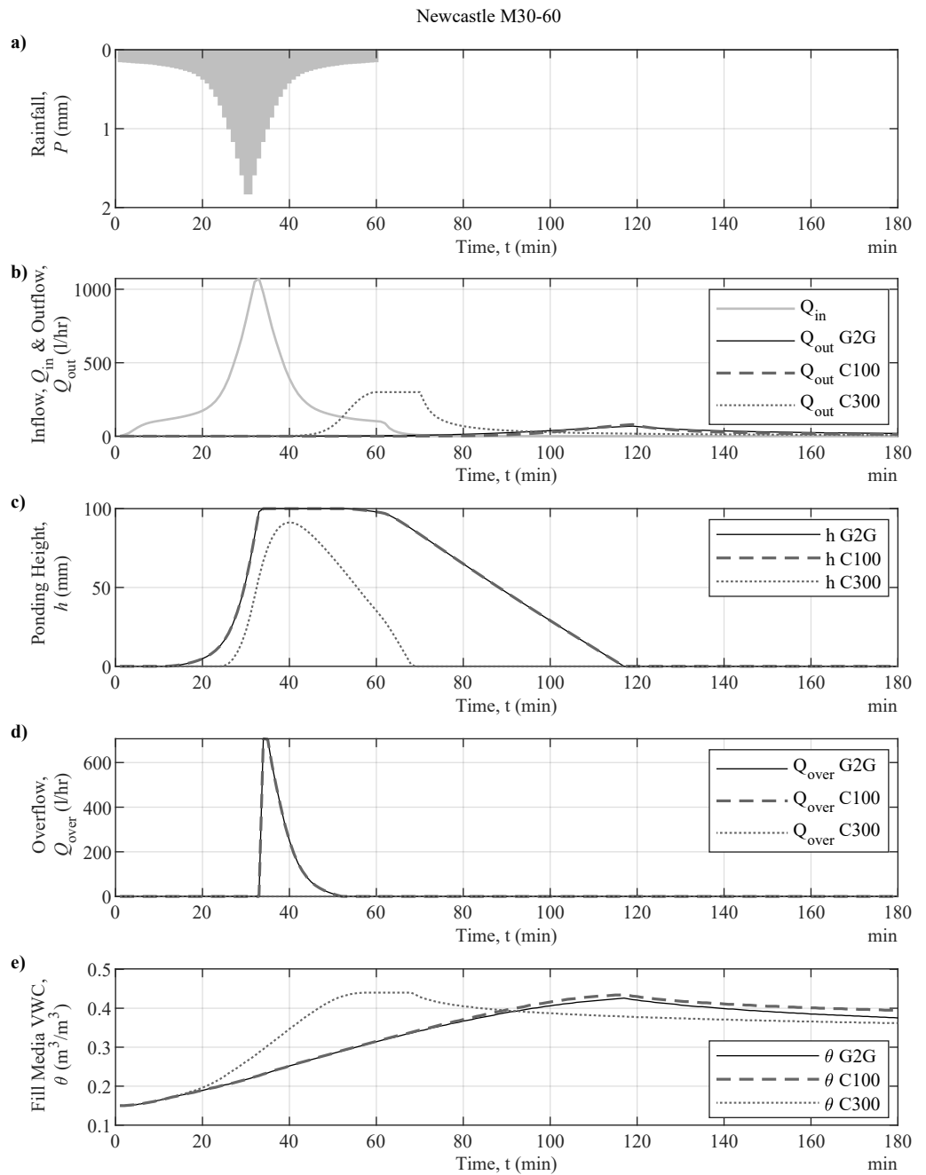
Figure A1. Modelled hydraulic response of bioretention systems in response to a 30-year return period 60-min duration storm event for Newcastle, UK. (a) Rainfall depth; (b) system inflow and outflow; (c) ponding height; (d) overflow; and (e) volumetric water Content (VWC) of the fill media.
