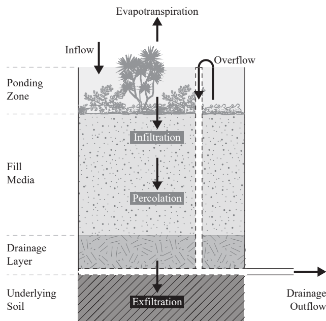
Figure 1. Schematic diagram of an unlined bioretention system with underdrain. Key hydrological processes are also indicated.
