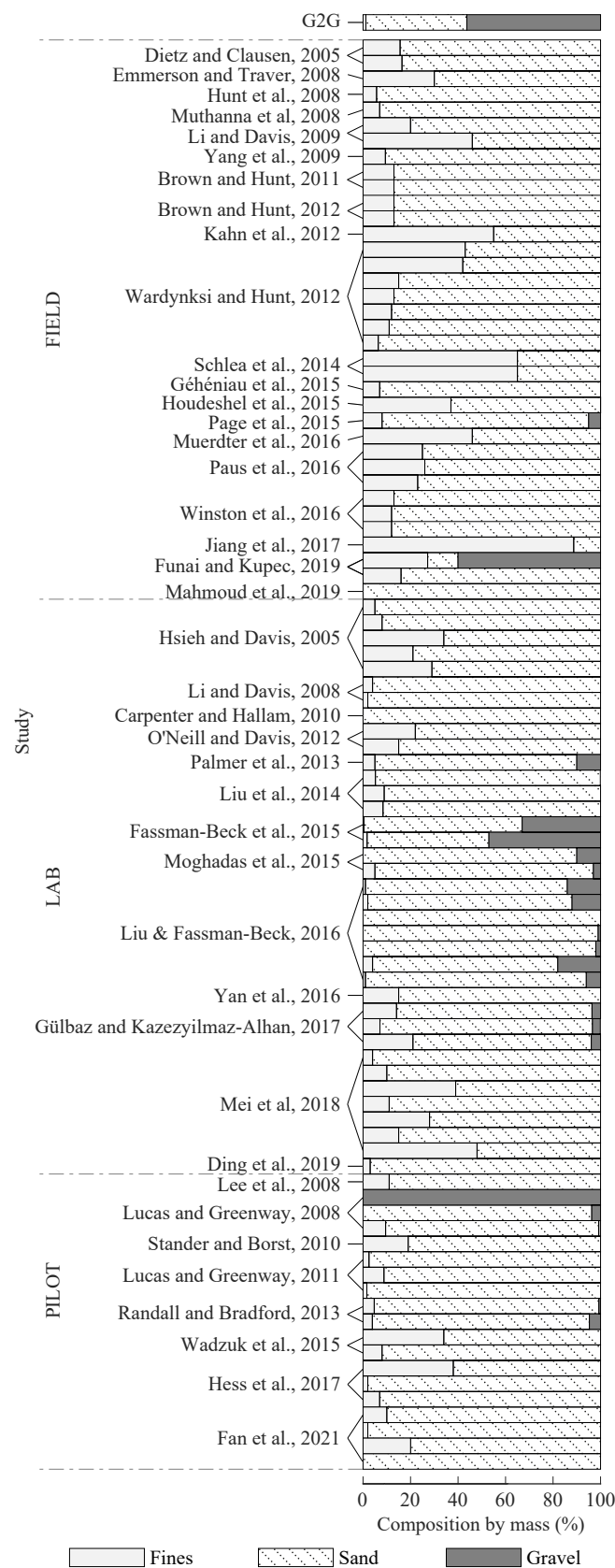
Figure 5. Comparison of G2G and literature examples of fill media composition by particle size class. Fines (<0.063 mm), sand (0.063–2.0 mm) and gravel (>2.0 mm).
