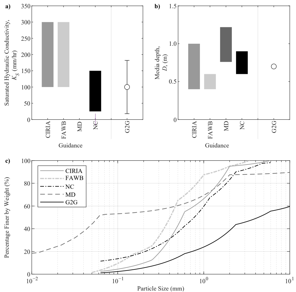
Figure 3. Comparison of G2G and Guidance Document ranges for: (a) Saturated Hydraulic Conductivity, with G2G plotted as mean \pm 1 standard deviation; (b) media depth, with G2G plotted as a single value; and (c) particle size distribution (plotted at the middle of the allowable range; linear interpolation of data is presented on the logarithmic x -axis).
