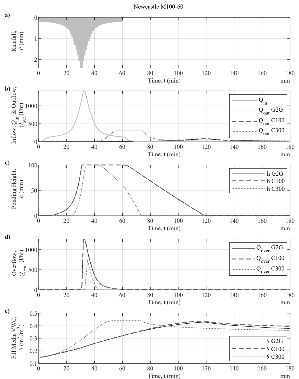
Figure A2. Modelled hydraulic response of bioretention systems in response to a 100-year return period 60-min duration storm event for Newcastle, UK. (a) Rainfall depth; (b) system inflow and outflow; (c) ponding height; (d) overflow; and (e) volumetric water content (VWC) of the fill media.
