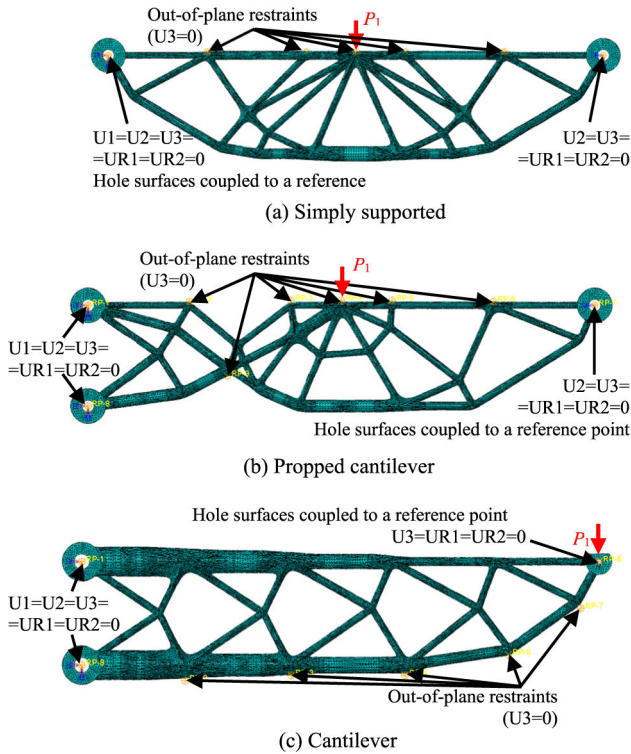
FIGURE 8. Boundary conditions of (a) simply supported, (b) propped cantilever and (c) cantilever trusses.
