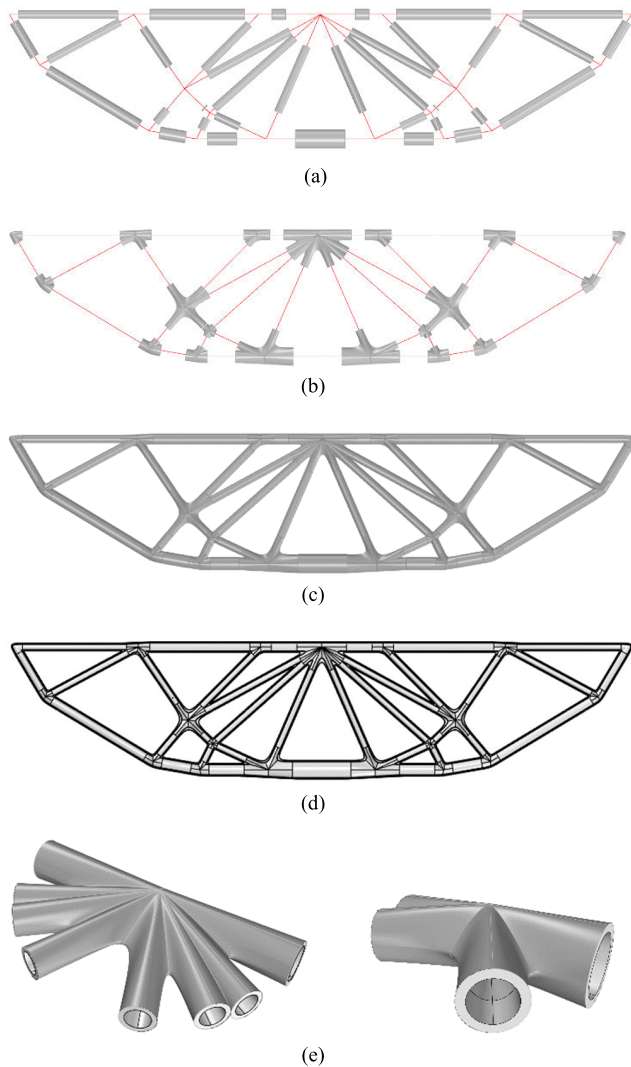
FIGURE 5. Generation of solid model of the simply supported optimized truss: (a) generation of circular members, (b) generation of connections between members, (c) finalised continuum truss, (d) section view of truss and (e) perspective view of typical joints.
