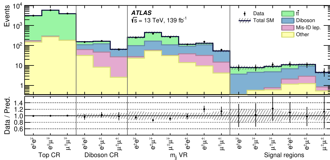
Fig. 5 The numbers of observed and expected events in the control, validation, and signal regions for all channels, split by lepton flavour and electric charge combination. The background expectation is the result of the background-only fit described in the text. The hatched bands include
