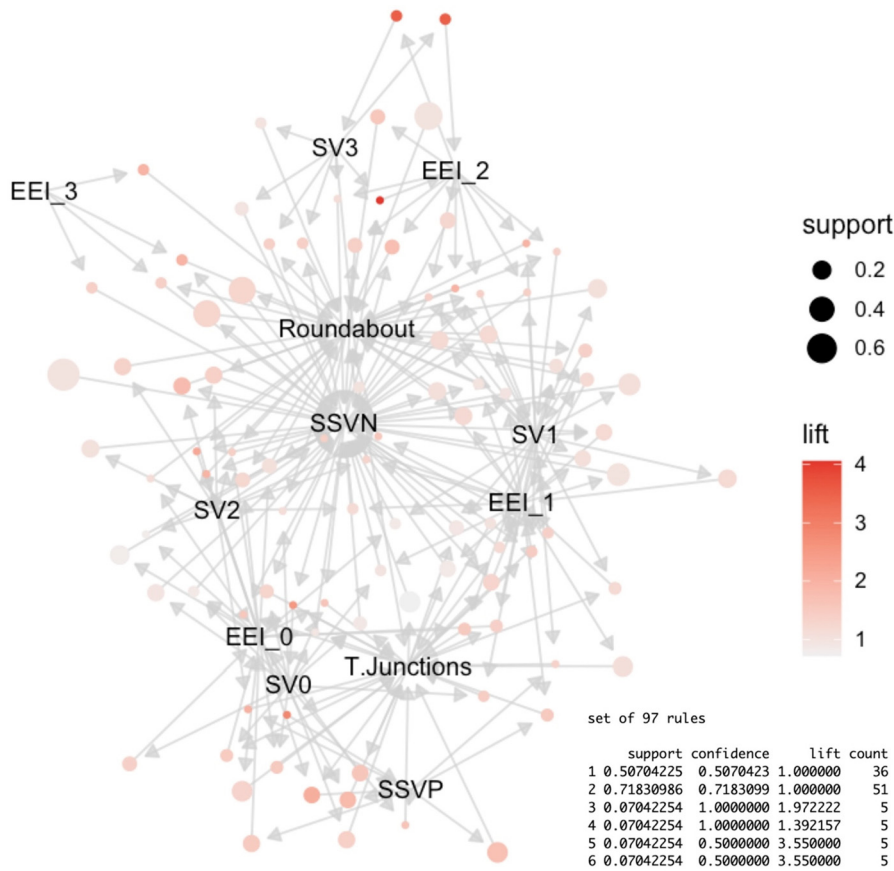
Fig. 7. Graph-based visualization with items and rules as vertices: plot shows the initial view of the complete graph. Legend: EEI ( Electrodermal Impact Index ): EEI_0 = No Peak; EEI_1 = Between 1 and 2; EEI_2 = Between 2 and 3; EEI_3 = Between 3 and 4. SV ( Speed Variation ): SV0 = Up to 10%; SV1 = Between 10% and 20%; SV2 = Between 20% and 30%; SV3 = Between 30% and 40%; SV4 = Between 40% and 50%; SV5 = Over 50%. SSV ( Sign of the Speed Variation ): SSVP = Positive sign (speed increase); SSVN = Negative sign (speed reduction).
