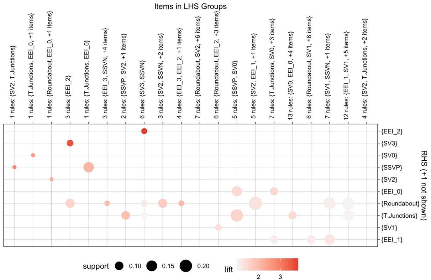
Fig. 9. Grouped matrix-based visualization with groups of antecedents in the columns and consequent items in the rows. Legend: EEI (Electrodermal Impact Index): EEI_0 = No Peak; EEI_1 = Between 1 and 2; EEI_2 = Between 2 and 3; EEI_3 = Between 3 and 4. SV (Speed Variation): SV0 = Up to 10%; SV1 = Between 10% and 20%; SV2 = Between 20% and 30%; SV3 = Between 30% and 40%; SV4 = Between 40% and 50%; SV5 = Over 50%. SSV (Sign of the Speed Variation): SSVP = Positive sign (speed increase); SSVN = Negative sign (speed reduction).
