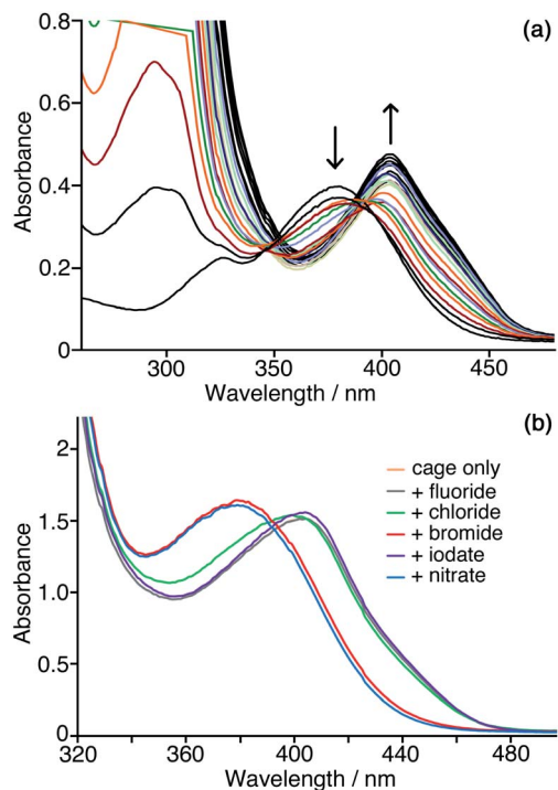
Fig. 6 Interaction of the CNP anion with the cage surface. (a) Addition of small samples (2 \mu\text{M} concentration increments) of H + to a solution of CNP (0.05 mM) in water, showing the red-shift in the CNP absorbance maximum as it binds to the cage surface; the red-shift of the maximum is complete after addition of ca. 0.3 equiv. of cage, thereafter only small changes in intensity occur. (b) Effects of addition different inorganic mono-anions (10 equiv.) to displace CNP from the surface of H + in water. Conditions: 0.05 mM H + and 0.1 mM CNP at pH 7. Note that the spectrum for 'cage only' (orange trace) is completely concealed under the spectrum recorded with added fluoride (purple trace), indicating the lack of ability of highly-solvated fluoride to displace CNP from the cage surface.
