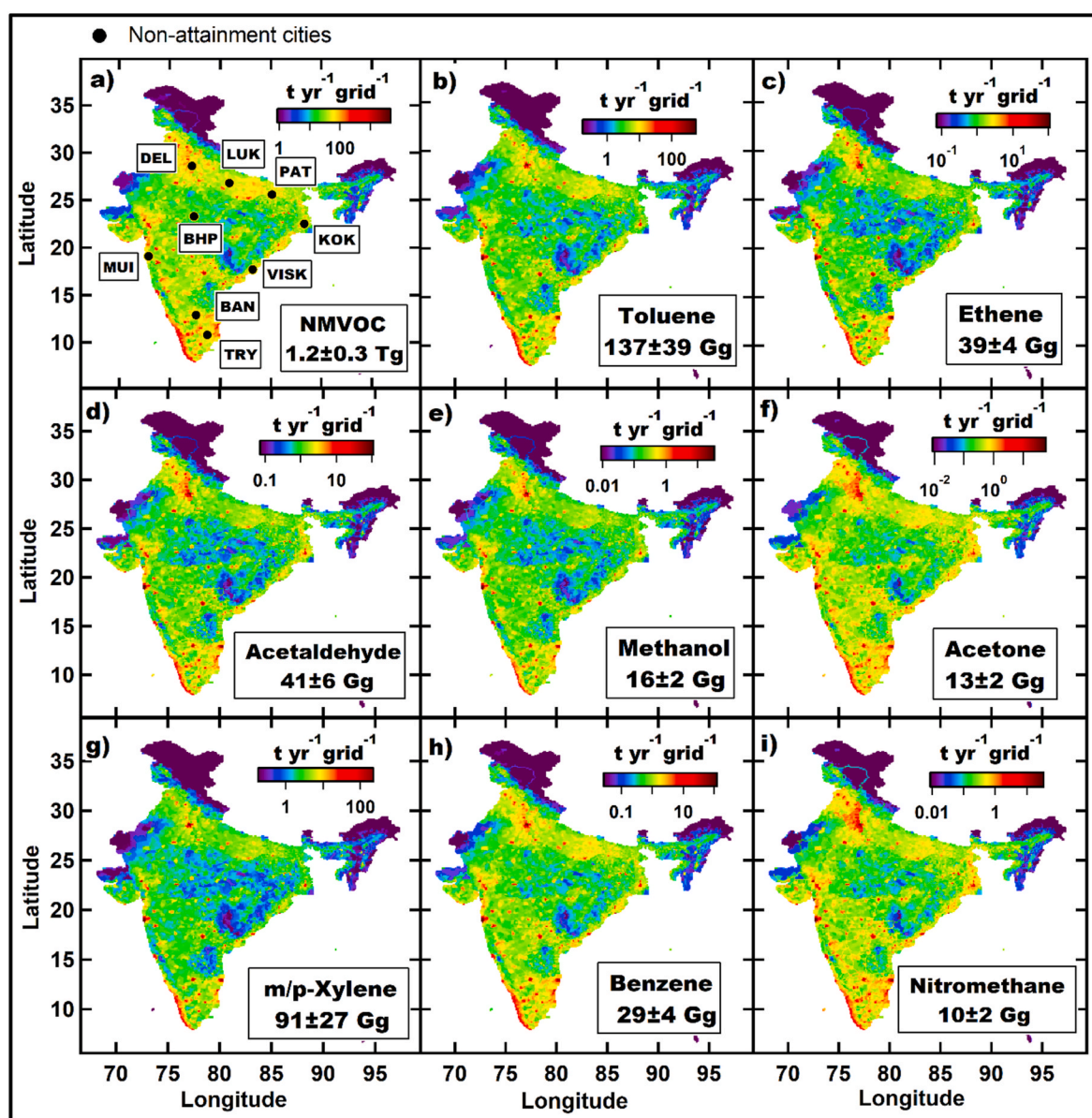
Fig. 3. Annual emissions of total NMVOC and selected VOC species from road transport sector in India for the year 2015–16. Markers indicate the location of major polluted cities identified by central pollution control board of India (CPCB) in which the prescribed national ambient air quality standard (NAAQS) limits are often violated (non-attainment cities). DEL – Delhi, LUK – Lucknow, PAT – PATNA, BHP – Bhopal, MUI – Mumbai, KOK – Kolkata, BAN – Bengaluru, VISK – Visakhapatnam, TRY – Trichy.
