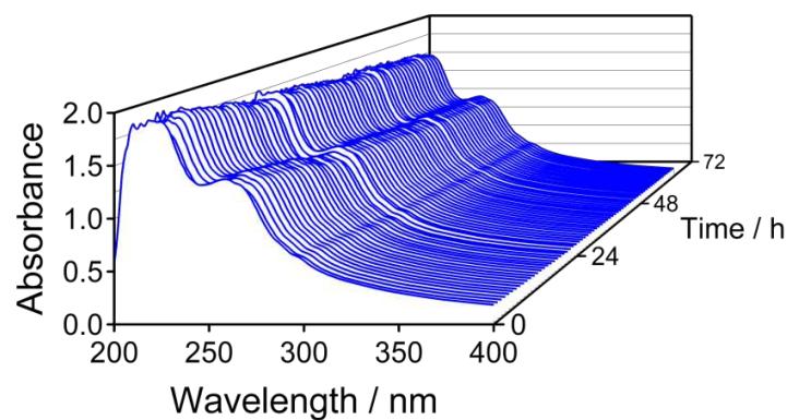
Figure S2. Series of UV-vis spectra of a suspension of 1 in \text{CH}_2\text{Cl}_2 over 72 h.
