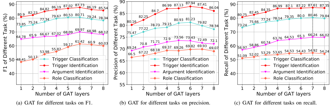
Fig. 5: The change of Precision, Recall and F1 for our model with different GAT layers under different tasks.
