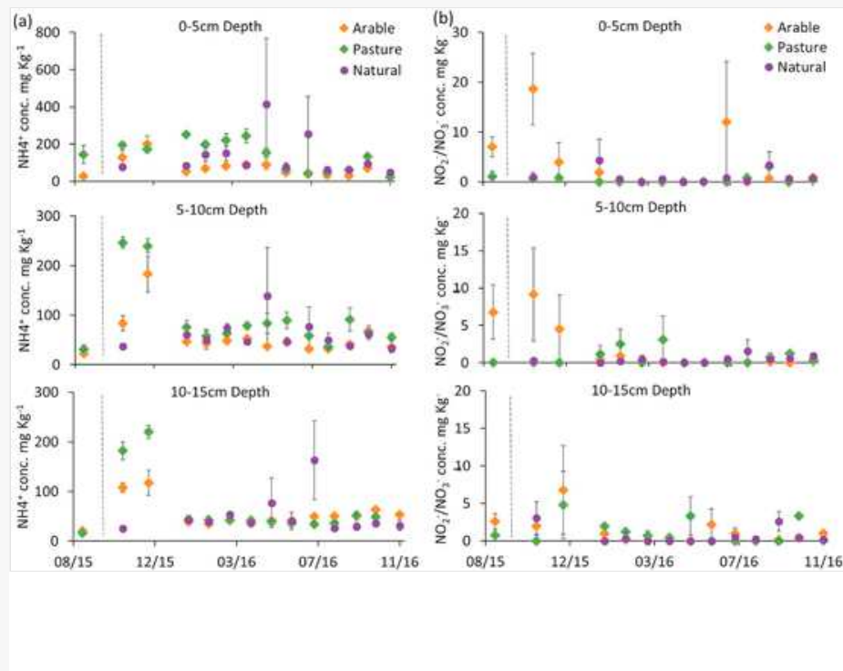
(a) Ammonium, \text{NH}_4^+ and (b) Nitrate/nitrite, \text{NO}_2^-/\text{NO}_3^- , concentration in sediment (mg/kg) over time at each depth in the natural and realigned fields. (Note the difference in scales for \text{NH}_4^+ and \text{NO}_x and the difference in scale in the 0–5 cm depth). Breach of sea wall (dotted line) was in Sept'15. Error bars are \pm\text{SE} , n = 4 .
