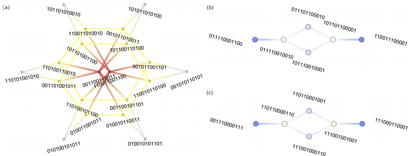
FIG. 3. Hilbert space fragmentation in a pair-hopping model in Eq. (24) studied in Ref. 72. Plots (a), (b) and (c) show graphs of three disconnected sectors of the Hilbert space for a small chain with N=6 electrons at filling factor \nu=1/2 . Each vertex represents a Fock basis state, and vertices are connected by an edge if the Hamiltonian matrix element is non-zero between those basis states. This type of graph is known as the adjacency graph of the Hamiltonian. In this case, because all the matrix elements of the Hamiltonian are equal in magnitude, the adjacency graph is unweighted. The graph has been coloured according to the vertex degree (with red colour indicating high connectivity).
