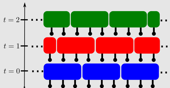
Figure B4: Illustration of the Floquet operator U^F = U^1 U^2 U^3 , staggered across three layers from Ref. 18.
