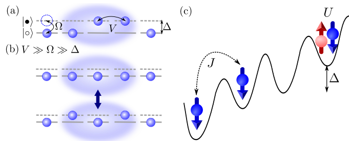
FIG. 7. (a) Rydberg atom as a two level system, where the empty circle corresponds to the ground state and the filled circle denotes the excited Rydberg state. The Rabi frequency is denoted as \Omega and the detuning of the |\bullet\rangle state from resonance is \Delta . The Rydberg blockade (shaded) leads to a shift of the energy level where both atoms are in the |\bullet\rangle -state, bringing it strongly off-resonance. (b) When the Rydberg blockade is strong ( V \gg \Omega \gg \Delta ), excitations of neighbouring atoms are energetically suppressed. In this limit, the effective model describing the Rydberg atom chain is the PXP model in Eq. (35). (c) Fermi-Hubbard model realised in an optical lattice 21 , with nearest neighbour hopping J and on-site interaction U . Tilt of the lattice is controlled by parameter \Delta [with a different meaning from the detuning \Delta in (a)-(b) and Eq. (45)!].
