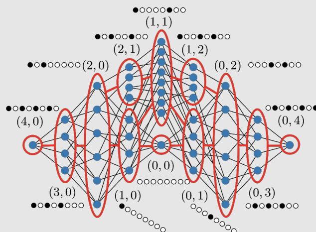
Figure B8: Construction of the symmetric subspace \mathcal{K} in the PXP model for L=8 spins. Each blue dot represents an allowed product state compatible with the constraint. The states are grouped into equivalence classes, denoted by ellipses. Each class is labelled by a representative state, e.g., the class (0,3) contains the representative state \bullet\bullet\bullet\bullet\bullet\bullet\bullet\bullet and all other obtained by permuting sites in each of the two sublattices. Reproduced from Ref. 132 under a Creative Commons licence CC BY 4.0.
