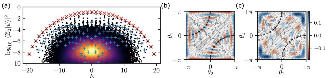
FIG. 6. (a) Scatter plot showing energies of all eigenstates of the PXP model vs. their overlap with |\mathbb{Z}_2\rangle state. Red crosses denote top-band quasimodes, blue pluses are the remaining quasimodes. Both of types of quasimodes are obtained by projecting the PXP model into the symmetric subspace \mathcal{K} defined in the text. Colour indicates the density of data points. (b)-(c): Viewing a selected top-band (b) and non top-band (c) quasimode as wavefunctions over \theta_1 and \theta_2 for L=128 . Colour scale represents the real part of the wavefunction. Top-band quasimodes concentrate around the classical periodic orbit (black line), displaying quantum scarring. The other quasimodes avoid this periodic trajectory and concentrate around the corners of the square. Note that the |\mathbb{Z}_2\rangle and its translated partner correspond to (\theta_1, \theta_2)=(\pi, 0) and (0, \pi) in the notation of this figure. Due to the MPS parametrisation, the wavefunction in (b) visibly spreads out towards the boundary and becomes completely delocalised at the edges, \theta_i = \pm\pi , where the points are indistinguishable in the transverse direction. Panels reproduced from Ref. 132 under a Creative Commons licence CC BY 4.0.
