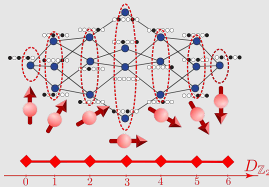
Figure B7: Graph representation of the PXP Hamiltonian for L=6 spins. Vertices represent all states compatible with the constraint, while lines connect states related by a single spin flip. The FSA models the non-thermal eigenstates and revivals from |\mathbb{Z}_2\rangle state by compressing the graph to a one-dimensional ladder of states, which are identified with basis states of a large spin of magnitude s = \frac{L}{2} (red arrows). The states are labelled by their z -projection of spin or, equivalently, by their Hamming distance D_{\mathbb{Z}_2} from the leftmost vertex.
