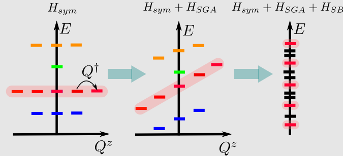
Figure B3: Tunnels-to-towers scheme for constructing non-thermal eigenstates from Ref. 68.
