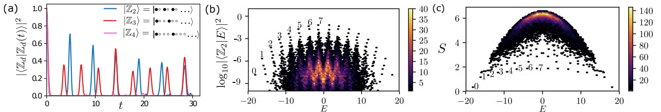
FIG. 4. (a) Numerical simulation of quantum fidelity in a large PXP model with L=30 atoms reveals strong atypicality with respect to the initial state 94 . For period-2 and -3 density waves, the fidelity features robust revivals, while period-4 density wave shows no revivals. (b)-(c): Non-thermal eigenstates violate the ETH by their anomalously large projection on |\mathbb{Z}_2\rangle state, and by their low entanglement entropy, S 94 . Each point represents a single eigenstate with energy E in a large PXP chain with L=30 atoms. Scarred eigenstates have been numbered by 0, 1, \dots, 7 . Colour scale represents the density of data points. Panels reproduced with permission from Ref. 94 APS, under a Creative Commons licence CC BY 4.0.
