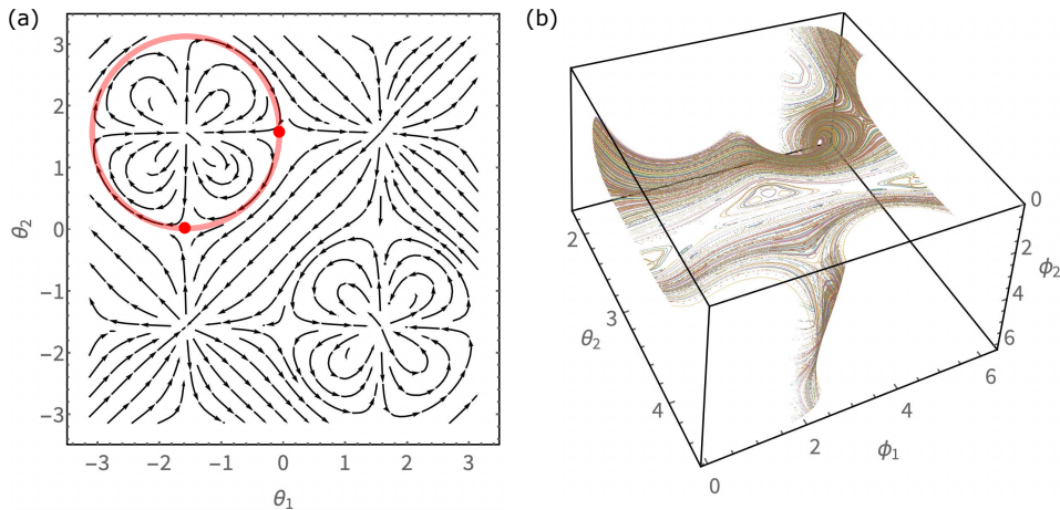
FIG. 5. (a) Flow diagram obtained from the variational ansatz with two degrees of freedom reveals an unstable periodic trajectory (red line), which is responsible for the fidelity revivals from the period-2 density wave state in the quantum case 14 . The periodic trajectory passes through the Néel states, |\mathbb{Z}_2\rangle and |\mathbb{Z}'\rangle , shown by red dots, and avoids the polarised state, |0\rangle \equiv |000\dots\rangle , located at (0,0) . As shown in Ref. 14, quantum leakage outside the variational manifold is minimised in the vicinity of the periodic orbit, thus explaining the relevance of this trajectory in the fully quantum dynamics. (b) In the presence of the chemical potential \mu_z \neq 0 , the dynamical system develops mixed phase space containing large regular regions, as shown in Ref. 97. The plot shows the associated Poincaré section for \mu_z = 0.325 at fixed (\theta_1^* = 1.25\pi, \dot{\theta}_1 < 0) .
