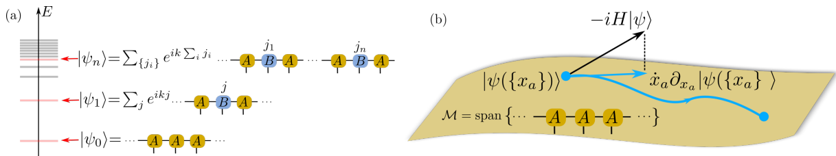
FIG. 2. MPS methods for weak ergodicity breaking. (a) Constructions of exact, highly-excited eigenstates using MPO-MPS techniques from Ref. 17. This method allows to construct a tower of quasiparticle states |\psi_n\rangle by acting with a local operator on the MPS ground state |\psi_0\rangle , as in Eq. (6) and (10). (b) Time-dependent variational principle captures the optimal projection of quantum dynamics onto a given variational manifold \mathcal{M} , here parametrised by MPS. Limiting the bond dimension of the MPS to be low, this approach defines a semiclassical limit for quantum dynamics. The corresponding classical system is formed by equations of motions for the coefficients x_a , which parametrise the projection of the wave function into the MPS manifold. The equations of motions follow from minimising the leakage outside the manifold, i.e., the deviation of -iH|\psi(t)\rangle from \dot{x}_a \partial_{x_a} |\psi(t)\rangle , see Eq. (14).
