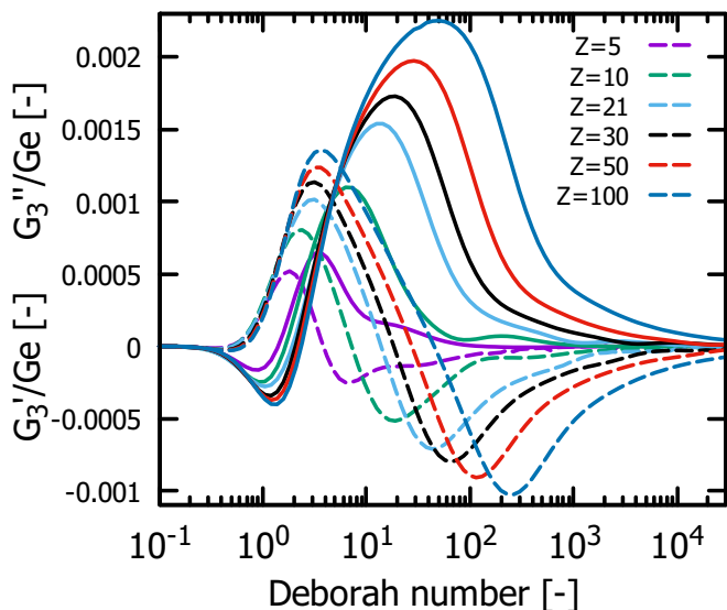
FIG. 4. GLaMM predictions of third harmonics with varied entanglement number. The solid lines are G_3' , and the dashed lines are G_3'' .
