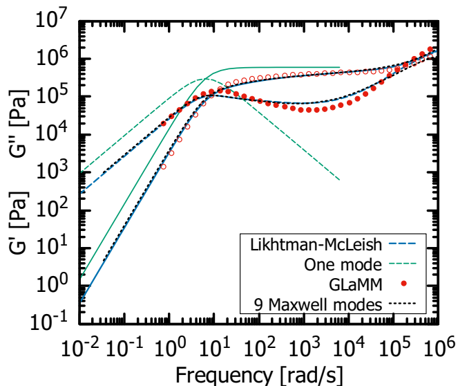
FIG. 2. Linear dynamic moduli predictions for PI100K at 25 °C, using Likhtman-McLeish theory, GLaMM, and Rolie-Poly with one and nine Maxwell modes. Details of the parameters used are provided in the Appendix.
