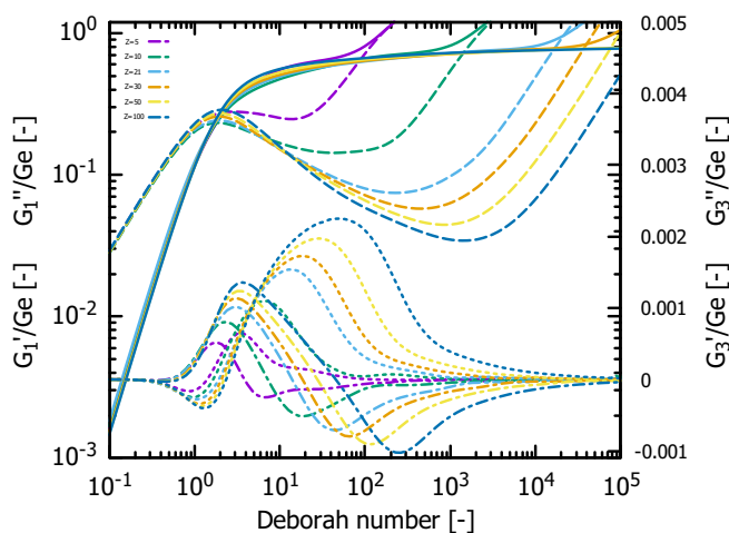
FIG. 5. Counterpart to Fig. 4. Variations in G_3' and G_3'' as a function of Z with comparison to the dynamic moduli. Of particular note is the characteristic crossover frequencies for each set of harmonics. In contrast to the experimental data the crossover for the third harmonics occurs at a higher frequency than the standard crossover.
