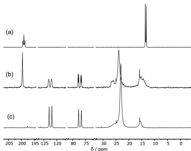
Figure 2. ^{31}\text{P}\{^1\text{H}\} NMR ( \text{THF-d}_8 , 25 °C, 203 MHz) showing reaction of [\text{Pd}_2^{\text{I}}(\mu\text{-PPh}_2)(\mu_2\text{-OAc})(\text{PPh}_3)_2] 1 with n\text{PPh}_3 . (a) Authentic 1 ; (b) [\text{Pd}_2^{\text{I}}(\mu\text{-PPh}_2)(\mu_2\text{-OAc})(\text{PPh}_3)_2] 1 + 1 equiv of \text{PPh}_3 after 0.5 h; (c) [\text{Pd}_2^{\text{I}}(\mu\text{-PPh}_2)(\mu_2\text{-OAc})(\text{PPh}_3)_2] 1 + 2 equiv of \text{PPh}_3 after 0.5 h. Note: the spectral window has been shortened, as shown by the double diagonal lines on the chemical shift scale line.
