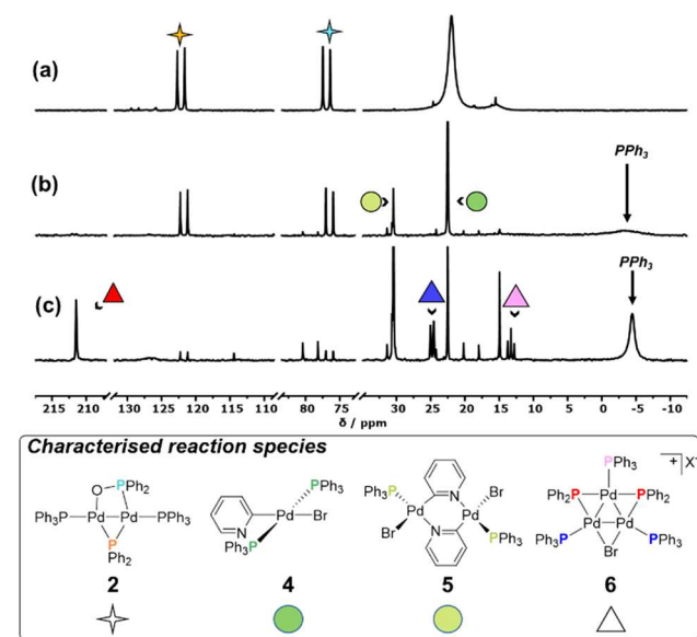
Figure 8. 31 P{ 1 H} NMR data (THF- d 8 , 25 °C, 203 MHz), recorded as a function of time, for the reaction between the postreaction mixture, generated from 1 and \text{PPh}_3 , and subsequent reaction with 2-bromopyridine. (a) before, (b) 20 min after, and (c) 13 h after addition of 2-bromopyridine.
