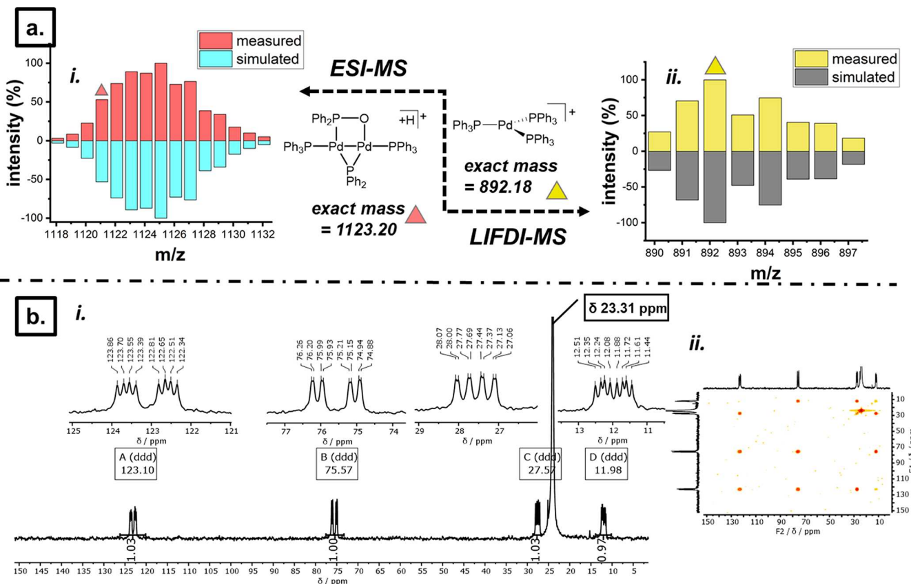
Figure 4. Key characterization data obtained from the postreaction solution (THF- d_8 ), containing the products of the reaction between [\text{Pd}^{\text{I}}_2(\mu\text{-PPh}_2)(\mu_2\text{-OAc})(\text{PPh}_3)_2] 1 and two equivalents of \text{PPh}_3 . (a) Mass spectral data for ions detected in the reaction solution; [\text{Pd}_2(\mu\text{-PPh}_2)\{\kappa_2\text{-P,O-}\mu\text{-P(O)Ph}_2\}(\text{PPh}_3)_2]^+ , detected by ESI-MS and [\text{Pd}^0(\text{PPh}_3)_3] detected by LIFDI-MS (right). (b) 1D ^{31}\text{P}\{^1\text{H}\} and 2D ^{31}\text{P}\text{-}^{31}\text{P}\{^1\text{H}\} COSY NMR spectra (202.5 MHz, \text{CD}_2\text{Cl}_2 ), recorded at 173 K of the postreaction solution.
