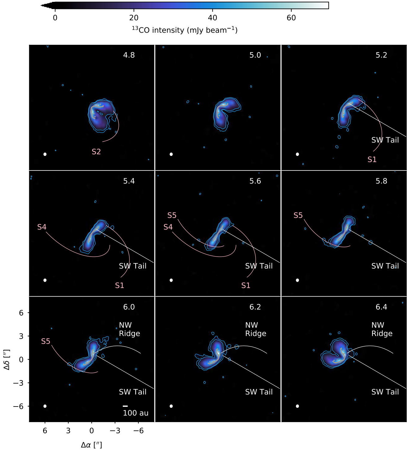
Figure 16. ^{13}\text{CO} J = 2 - 1 channel maps annotated with the locations of ^{12}\text{CO} features for which counterparts are tentatively identified in ^{13}\text{CO} . The blue contours mark the 4 and 8\sigma emission levels, where \sigma = 1 \text{ mJy beam}^{-1} . The Keplerian isovelocity contours are drawn in gray, with solid curves marking the front side of the disk and dashed curves marking the back side. The synthesized beam size, 0''.39 \times 0''.35 ( -4.4 ), is represented with a white ellipse in the lower left corner of each panel.
