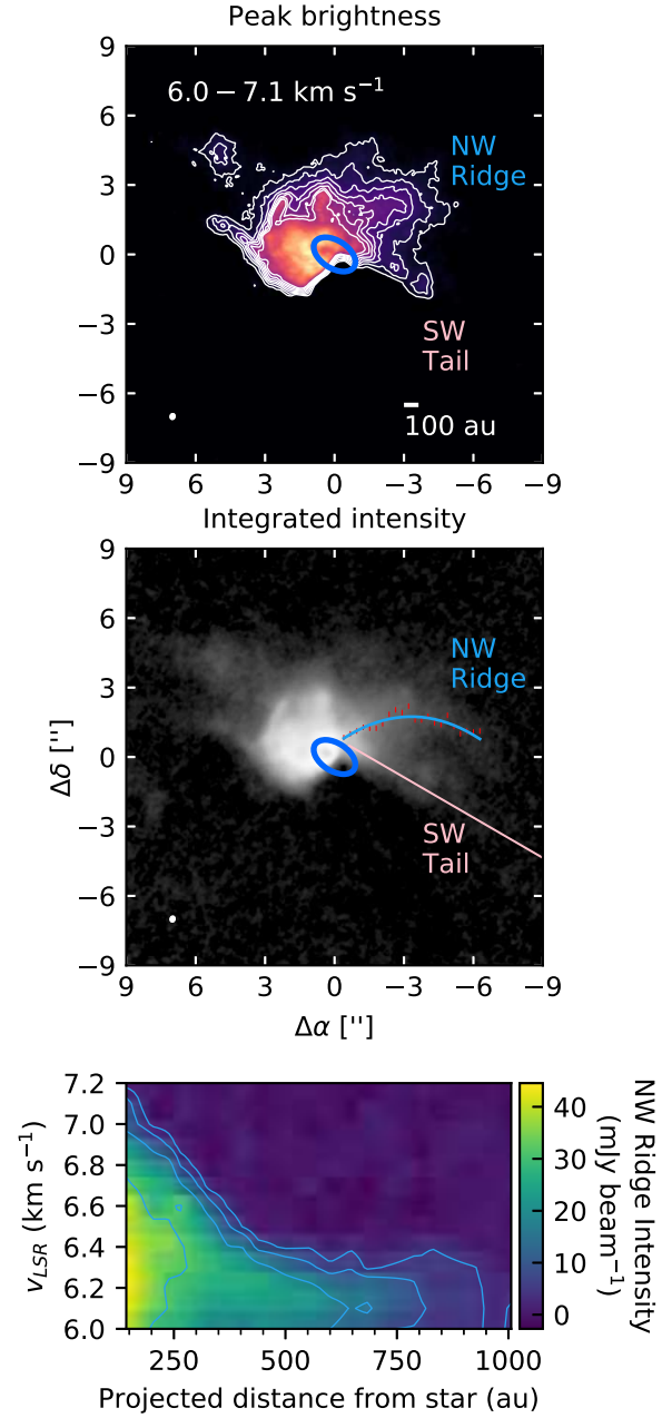
Figure 10. Top: A ^{12}\text{CO} peak brightness map from channels between 6.0 and 7.1 \text{km s}^{-1} , showing a broad “ridge” of emission northwest of the disk. The collimated component to the south is part of the southwest tail. Contours are drawn in increments of 5 \text{mJy beam}^{-1} , starting from 10 and ending at 40 \text{mJy beam}^{-1} . The blue ellipse shows the position angle and inclination of the GM Aur disk. Middle: The integrated intensity map from 6.0 to 7.1 \text{km s}^{-1} , with the measured positions of the local maxima along the northwest ridge and the 1\sigma error bars plotted in red. The best fit quadratic curve to the shape of the northwest ridge is drawn in light blue. The southwest tail is marked in pink. Bottom: Position-velocity diagram extracted along the best-fit curve to the northwest ridge. Contours are drawn at [4, 8, 16, 32] \text{mJy beam}^{-1} .
