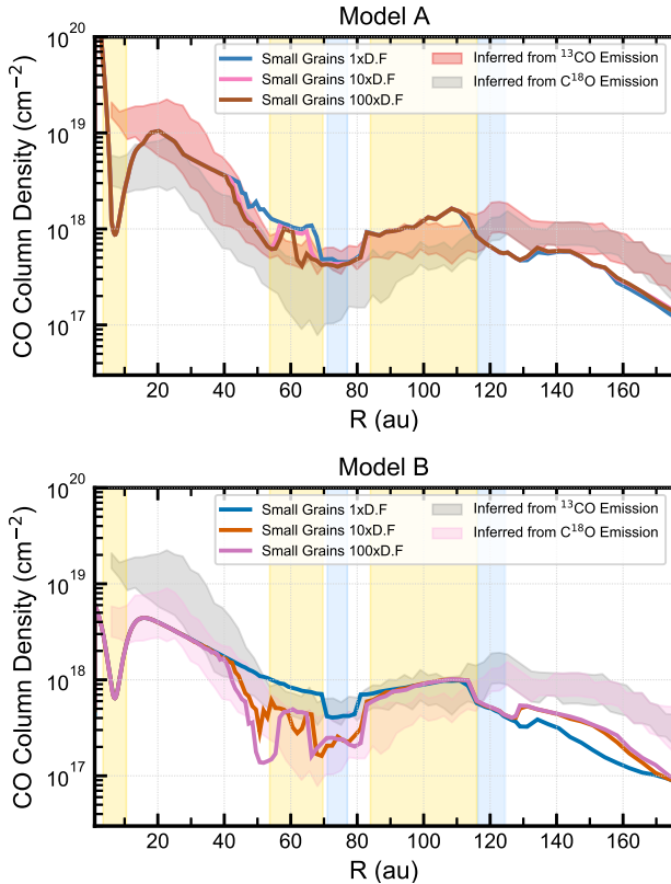
Figure 4. CO column-density profiles for both sets of simulations. Top: smooth gas surface density applying the CO depletion profile in Figure 2. Bottom: Simulation set with CO as a gas mass tracer. The vertical shaded areas are the location of dust substructures, while the radial shaded regions represent the CO column densities derived in Zhang et al. (2021) using ^{13}\text{CO} and \text{C}^{18}\text{O} emission. In both cases, Models A and B, we observe that whether including CO chemical processing or the gas depletion match the recovered CO column densities. The shaded regions are the locations of the dust gaps and dust rings, in yellow and blue, respectively.
