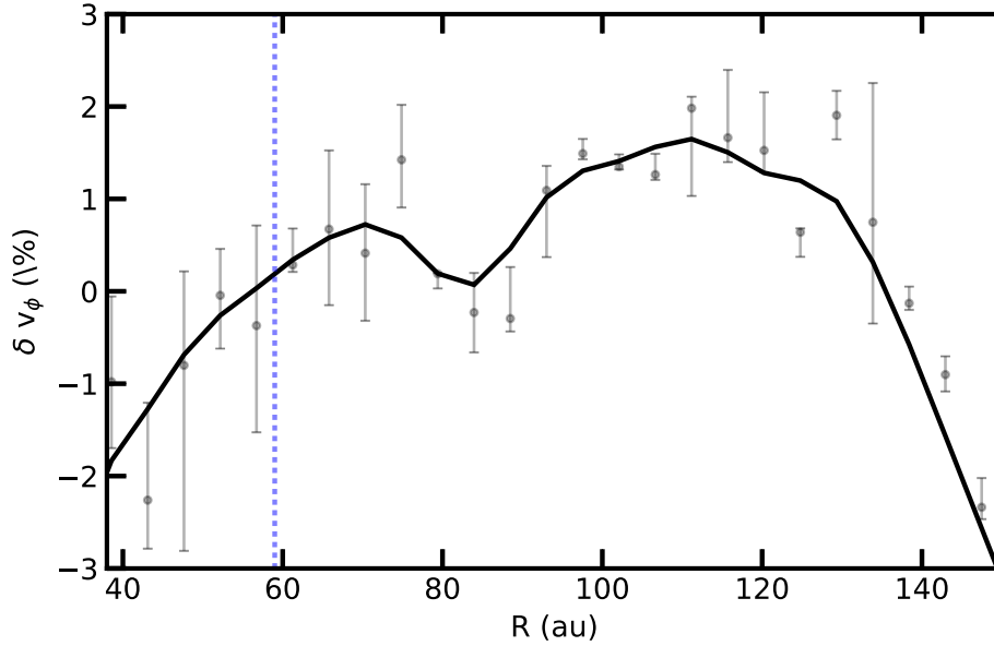
Figure 17. Kinematic deviations in the AS 209 disk using the CO data from MAPS (Oberg et al. 2021). The deviations show variations < 1\% at the location of the CO column-density gap, which is illustrated by the vertical dotted line. The continuous profile is the expected profile through a convolution with a 0''.15 resolution ( \sim 18 au). The recovered deviations seem consistent with the profile obtained by Teague et al. (2018) with lower-resolution data, reassuring that the kinematic deviation in AS 209 is not strong enough to cause a deep gas gap at 59 au.
