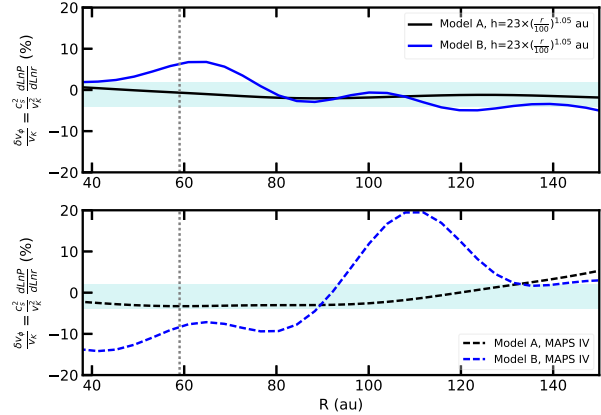
Figure 7. Expected velocity deviations in our models inferred from the pressure profiles. We inferred the velocity deviations using the relationships described by Rosotti et al. (2020) . The shaded area illustrates the range of kinematic deviations from the data (see Appendix C). In Model A the deviations are significantly smaller than in Model B. Model A does not present strong kinematic deviations from its pressure profile, while Model B with a gas gap shows deviations of the order of 10% in both surfaces.
