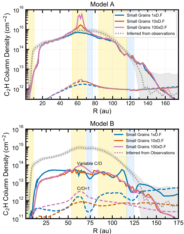
Figure 9. C_2H column-density profiles compared with the inferred values from observations. Top: simulation set for Model A. Bottom: simulation Set for Model B. The shaded areas in yellow and blue are the dust gaps and dust ring, respectively. Variable C/O models are shown in continuous lines, while the dashed lines are the models with a constant C/O ratio equal to 1. Our simulations show that depleting the number of small dust grains increases the C_2H column density by a factor of a few. However the main player in the C_2H column density is the C/O ratio.
