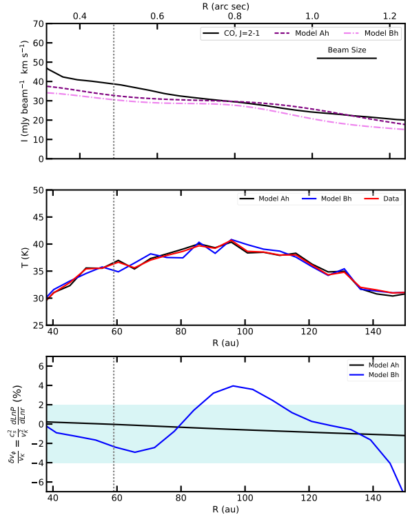
Figure 8. Comparison of data and expected values of thermochemical models with three iterations of hydrostatic equilibrium. Top: CO J = 2 - 1 emission profile. Middle: thermal cuts for both models matching the brightness temperature of the CO J = 2 - 1 line (Law et al. 2021a). Bottom: expected kinematic deviations in Models Ah and Bh with the range from the observations represented by the shaded area. The models show that the CO J = 2 - 1 is, to a small uncertainty, well traced in both cases. The kinematic deviations in Models Ah and Bh show that even when a few iterations of hydrostatic equilibrium are considered, the results stand, i.e., the kinematic deviations in Model Bh with a \text{H}_2 gas depletion are stronger and cover a larger range than the ones observed in the data.
