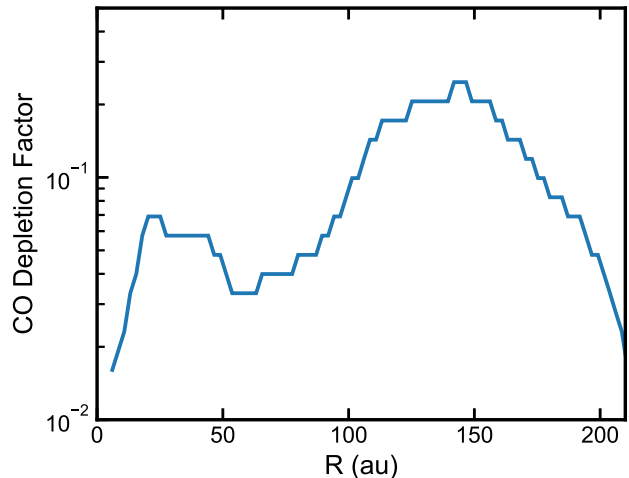
Figure 2. CO depletion used in Model A to fit the CO intensity profile. This depletion is used to compare the case with CO chemical processing (Model A) and the case with CO used as a tracer of \text{H}_2 surface density (Model B).
