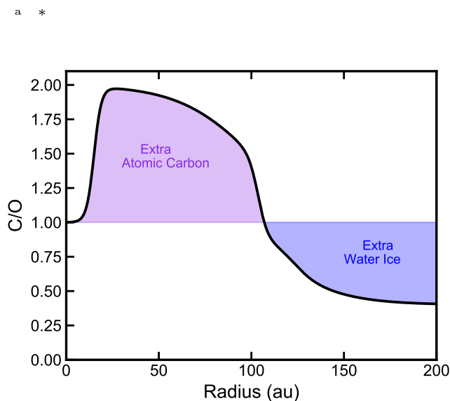
Figure 3. C/O ratio for our models with radial changes in the amount of C. The C/O starts at 1, then it reaches a value of 2 in the gas gap where extra atomic carbon is added. In this region most of the carbon grain destruction would occur. It also coincides with the region where the C_2H column density reaches its highest values. Beyond 100 au we added extra water ice to decrease the C/O ratio toward an ISM value C/O=0.4 .
