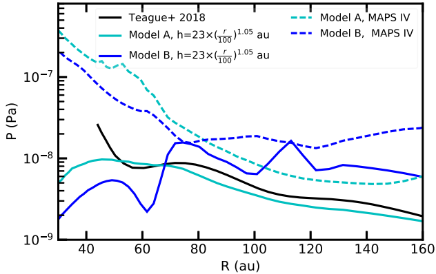
Figure 6. Thermal pressure profile cuts in our two models compared to the profile from Teague et al. (2018) inferred from AS 209 disk kinematics using CO line emission. The other cut was taken following the parametric emission surface of CO inferred by Law et al. (2021b) . When the gas is depleted by roughly an order of magnitude, as in Model B, the pressure profile shows significant variations with the radius, these are inconsistent with those from Teague et al. (2018) . The lack of strong fluctuations in the observed pressure profile disfavors the presence of a deep gas gap, at least at \sim 59 au, breaking the degeneracy between chemical processing and gas depletion. Thus, chemical processing is the dominant mechanism for CO column variations in AS 209.
