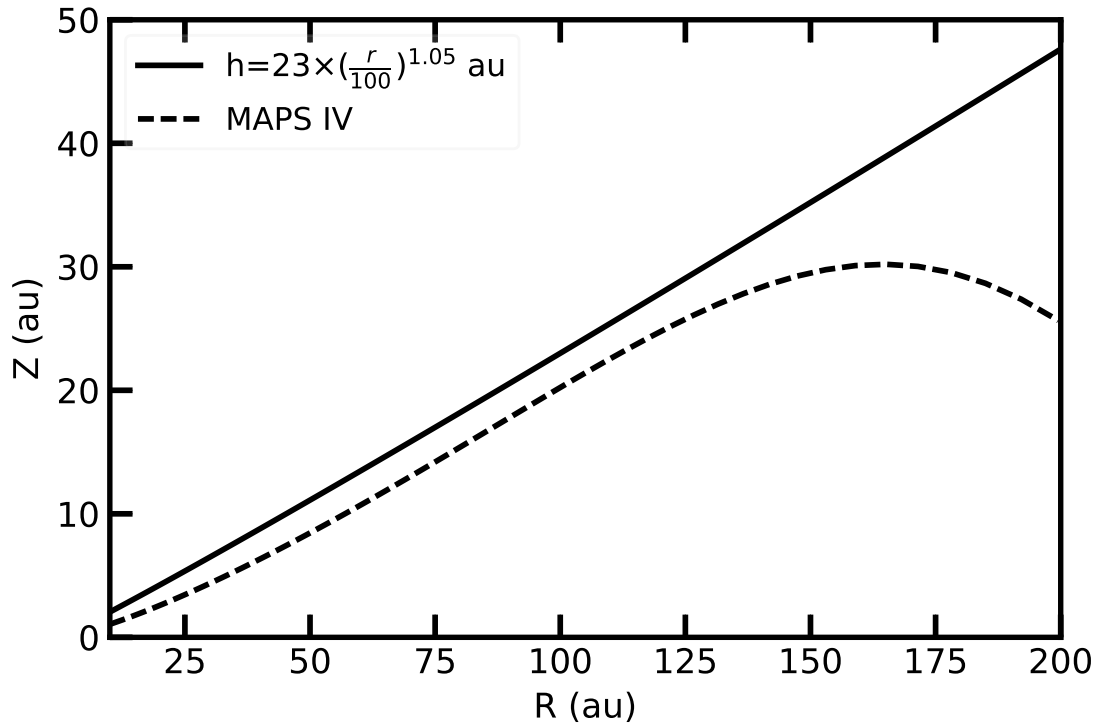
Figure 16. Emission heights found by Teague et al. (2018) and Law et al. (2021b) for the CO J = 2 - 1 emission coming from the AS 209 disk. These surfaces were used to extract the Keplerian deviation in our models and compare them with the observational ones.
