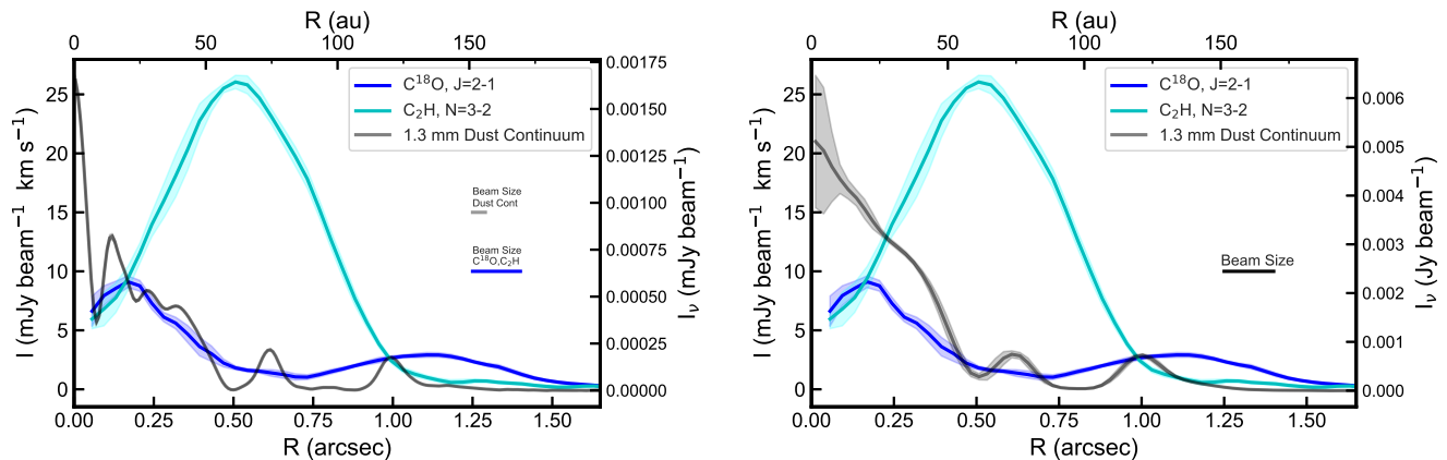
Figure 11. C_2H and C^{18}O radial profile for the velocity-integrated emission lines in ALMA Band 6, while the gray line displays the continuum-emission profile from DSHARP (Andrews et al. 2018; Guzmán et al. 2018) on the left and from MAPS (Oberget al. 2021) on the right. We observe that C^{18}O shows a wide gap before showing a second peak after the outer ring at 120 au. C_2H shows an inverse correlation to C^{18}O , peaking at the location of the C^{18}O gap, making AS 209 a unique source for the study of CO chemical processing among the sources in the MAPS survey.
