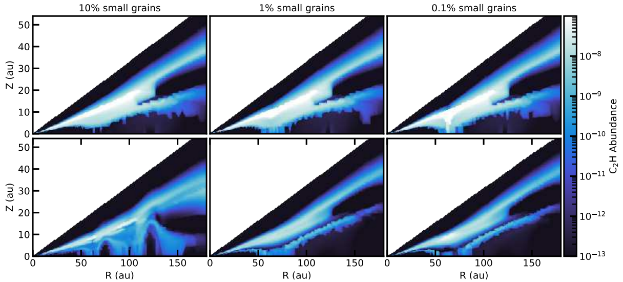
Figure 15. C 2 H 2D abundance structure in each set of simulations. Top row: C 2 H abundance structure for Model A. Bottom row: C 2 H abundance structure for Model B. In the regions where the small dust is depleted, C 2 H can be produced closer to the midplane. This causes the slight increases in C 2 H column density observed in Fig. 9.
