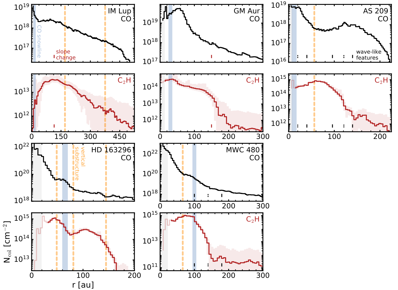
Figure 14. Column density profiles for CO (Zhang et al. 2021) and C 2 H (Guzmán et al. 2021) for all MAPS sources versus locations of vertical substructures in CO, 13 CO, and C 18 O 2–1 emission lines. Orange dashed lines indicates vertical dips listed in Table 4. The CO snowlines from Zhang et al. (2021) are shaded in blue. Red solid lines indicate the radial locations of changes in emission surface slope. The low-amplitude, wave-like features in AS 209 and MWC 480 are shown in black with dashed and solid lines marking troughs and peaks, respectively.
