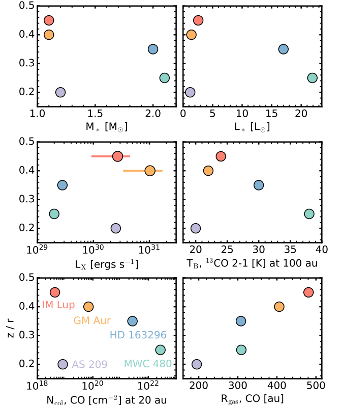
Figure 13. Average z/r of ^{12}CO 2–1 emission heights versus disk physical properties for the MAPS sources. Stellar masses and bolometric luminosities, taken from Oberg et al. (2021) and references therein, while X-ray luminosities references are: IM Lup (Cleeves et al. 2017), AS 209 (Walter & Kuhl 1981), GM Aur (Espaillat et al. 2019), HD 163296 (Günther & Schmitt 2009), and MWC 480 (Grady et al. 2010). Horizontal bars indicate observed intrinsic X-ray variability. Brightness temperatures of ^{13}CO 2–1 at 100 au are interpolated directly from the T_B radial profiles in Figure 7, so they sometimes differ from the fitted T_{100} in Table 2. If we instead adopted the fitted T_{100} values, the conclusions are unchanged. Peak CO column densities are from Zhang et al. (2021) (and see Figure 14), while the CO 2–1 disk sizes are from Law et al. (2021).
