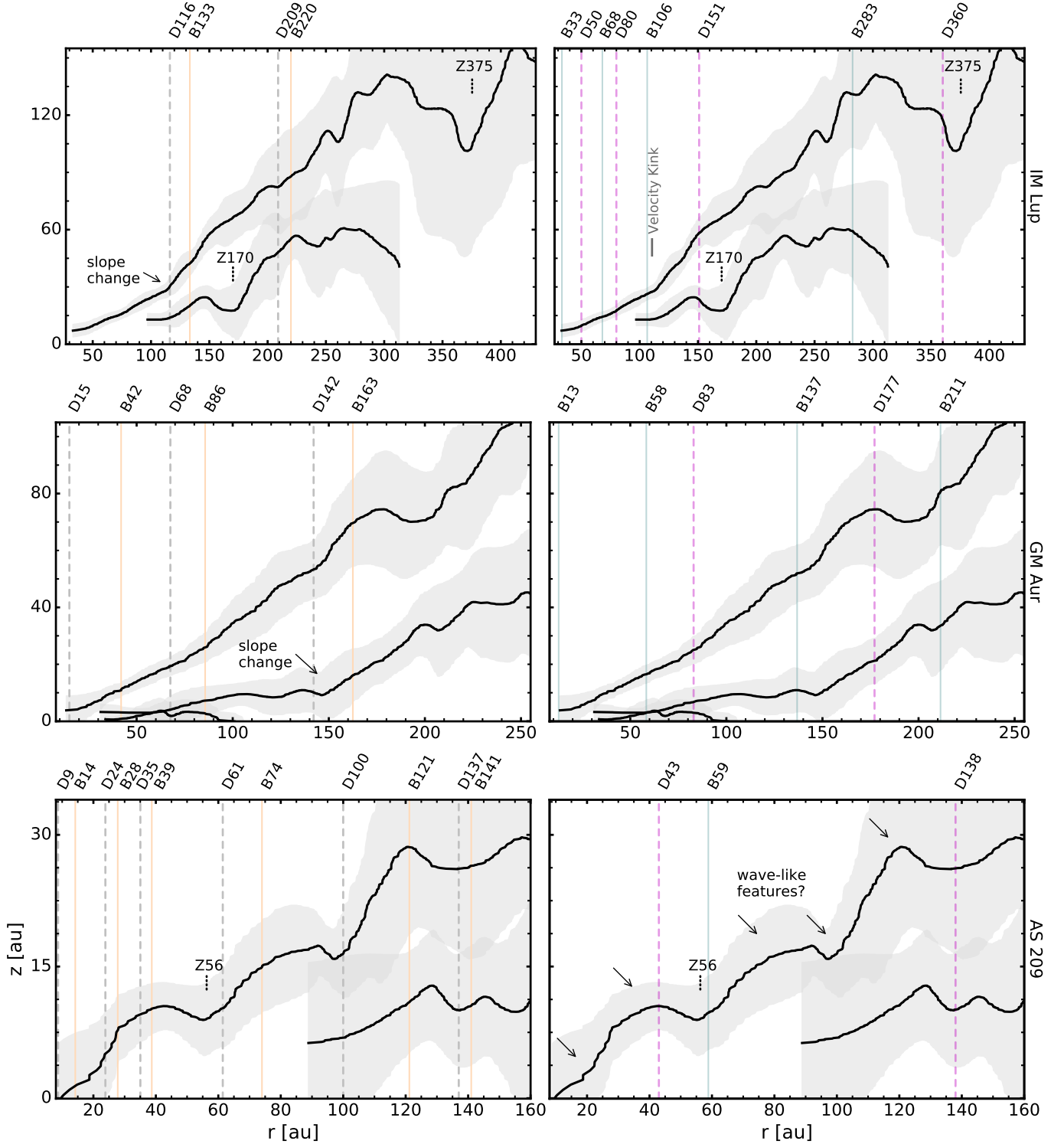
Figure 12. Comparison of CO 2–1, ^{13}\text{CO} 2–1, and \text{C}^{18}\text{O} 2–1 (when available) surfaces with annular substructures in the millimeter continuum (left) and CO line emission (right). Substructures are labeled following the nomenclature of Huang et al. (2018) and taken from Law et al. (2021). The CO line emission substructures are from CO 2–1 for all disks, except for MWC 480, which show those from ^{13}\text{CO} 2–1. Substructures are labeled as follows: dust ring (solid orange line), dust gap (dashed gray line), and chemical gap (dashed purple line). Dotted black lines mark vertical substructures, as listed in Table 4. Notable changes in emitting surface slope and the suggestive wave-like features in AS 209 and MWC 480 are marked with arrows. The CO velocity kinks from Pinte et al. (2018, 2020) are labeled in IM Lup and HD 163296.
