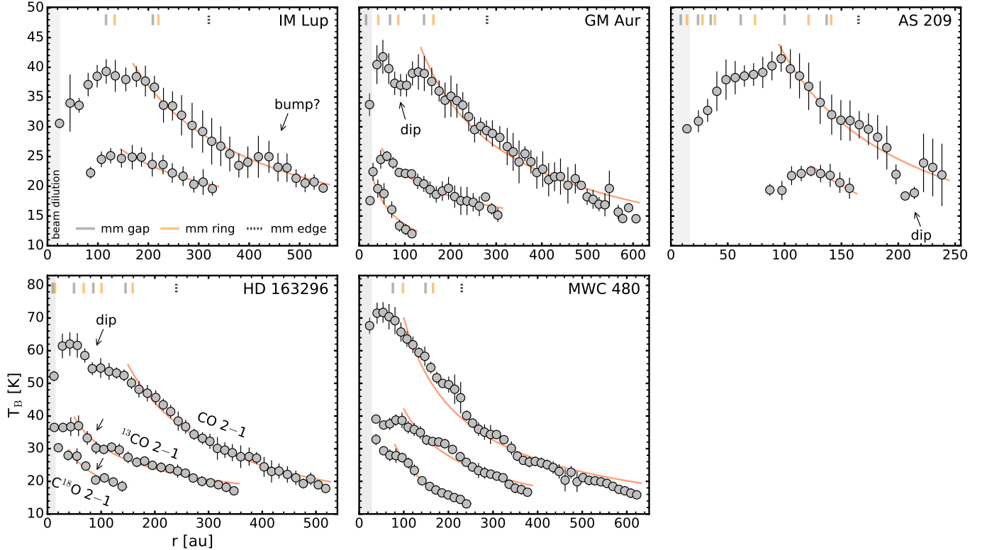
Figure 7. Radial brightness temperature profiles for CO 2–1, ^{13}\text{CO} 2–1, and when available, \text{C}^{18}\text{O} 2–1. The top and bottom rows are each shown on a consistent temperature scale and are grouped by whether the host star is a T Tauri or Herbig Ae star, respectively. These profiles represent the mean temperatures computed by radially binning the individual measurements, similar to the procedure used to compute the radially-binned surfaces (see Section 4.3.1). Vertical lines show the 1\sigma uncertainty, given as the standard deviation of the individual measurements in each bin. For increased visual clarity, all disks have been binned by an extra factor of two, except for IM Lup and HD 163296, which have been binned by an additional factor of three and four, respectively. The solid red line shows the fitted power law profile from Table 2. The inner gray shaded region is the FWHM of beam major axis. The orange and gray dashes correspond to the mm continuum rings and gaps, respectively. The black dots mark the outer edge of the millimeter continuum. Temperature dips in GM Aur, AS 209, and HD 163296 are labeled with arrows, as is a temperature bump in IM Lup.
