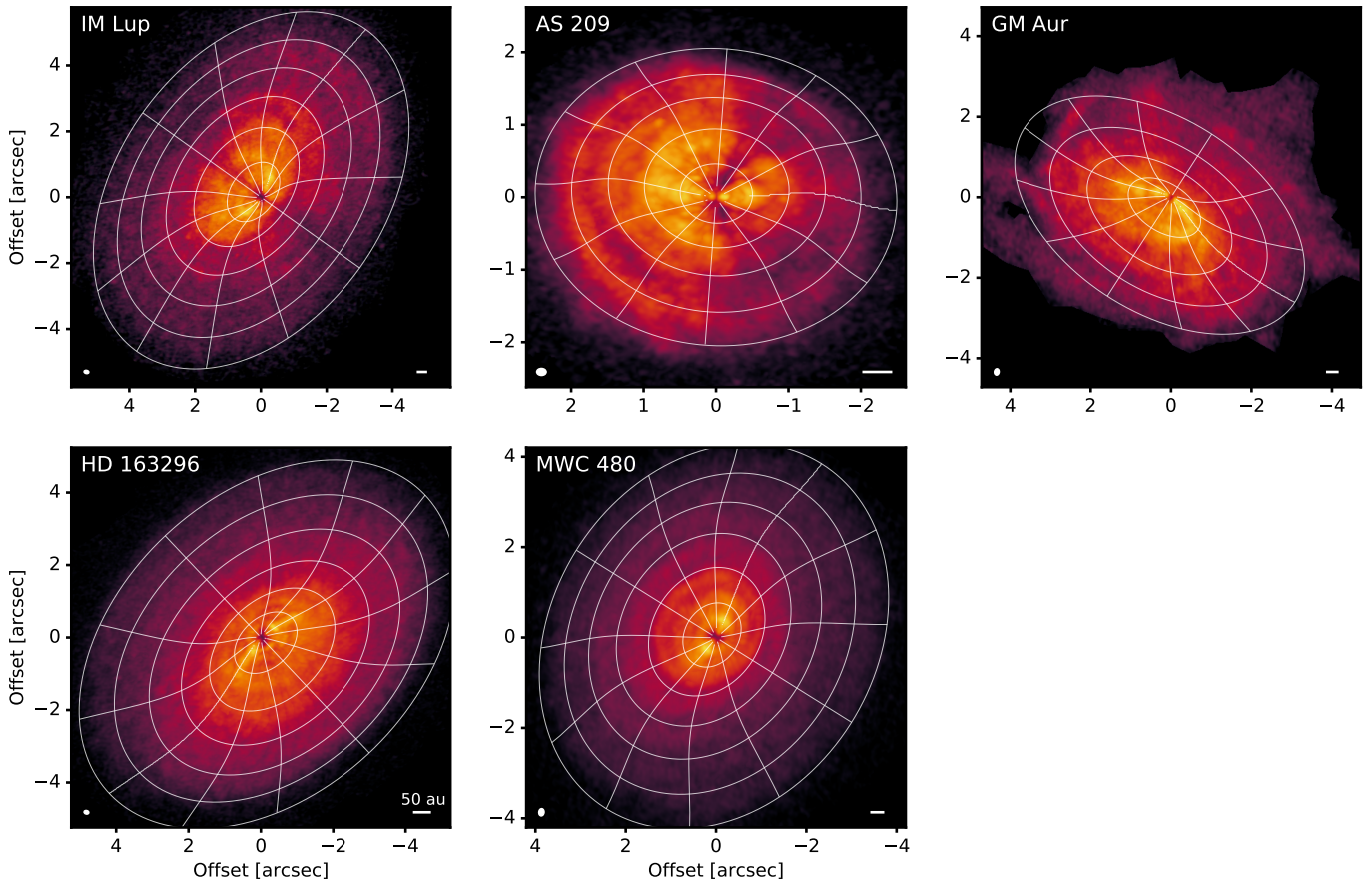
Figure 3. Peak intensity maps of CO 2–1 for all MAPS sources with overlaid contours showing the fitting emission surfaces, as listed in Table 1. The synthesized beam and a scale bar indicating 50 au is shown in the lower left and right corner, respectively, of each panel.
