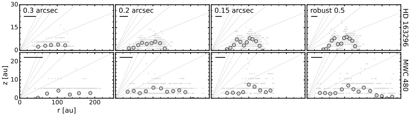
Figure 20. \text{C}^{18}\text{O} 2–1 emission surfaces derived using different spatial resolutions for HD 163296 and MWC 480. The \text{C}^{18}\text{O} 2–1 surface in GM Aur is not shown as it was only able to be extracted from the images generated with a robust parameter of 0.5, as only this image possessed a sufficiently high spatial resolution necessary to separate the front and back disk surfaces. Otherwise, as in Figure 18.
