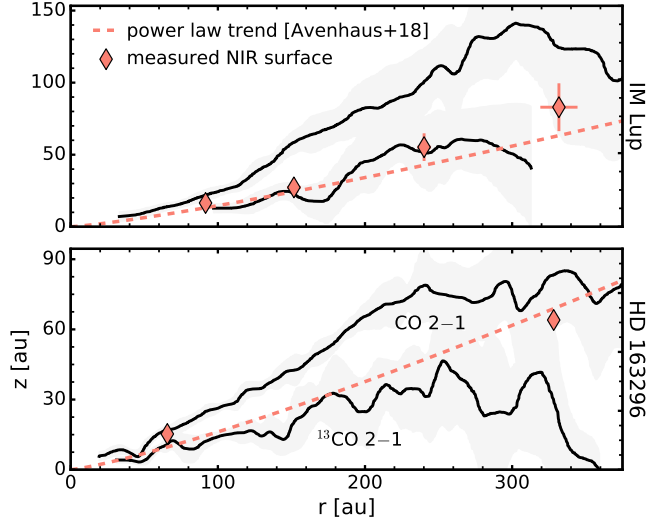
Figure 6. Emission surfaces of CO and 13 CO 2–1 in IM Lup (top) and HD 163296 (bottom). The black lines are the moving average surfaces and gray shaded regions show the 1\sigma uncertainty. The red diamonds show individual height measurements of NIR rings (Monnier et al. 2017; Avenhaus et al. 2018; Rich et al. 2020), while the red dashed line shows the inferred NIR surface using the relation found in a sample of disks in Avenhaus et al. (2018). The values from Monnier et al. (2017) have been scaled to reflect the updated Gaia distance for HD 163296. The errorbars are smaller than the marker for the innermost rings in both IM Lup and HD 163296 and the 330 au ring in HD 163296 does not have reported uncertainties.
