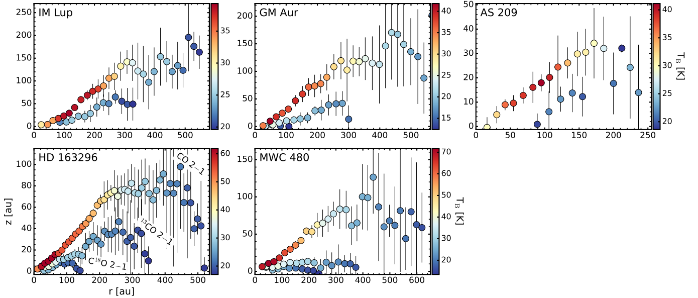
Figure 9. 2D temperature distributions of CO 2–1, ^{13}\text{CO} 2–1, and when available, \text{C}^{18}\text{O} 2–1 in all MAPS sources. Points are those from the binned surfaces and error bars are the 1\sigma uncertainties in z . For some of the innermost points, the uncertainty is smaller than the marker. Data for all disks and lines have been binned by a factor of three for visual clarity. The uncertainty of the temperature measurements, which is not shown here, can be found in Figure 7.
