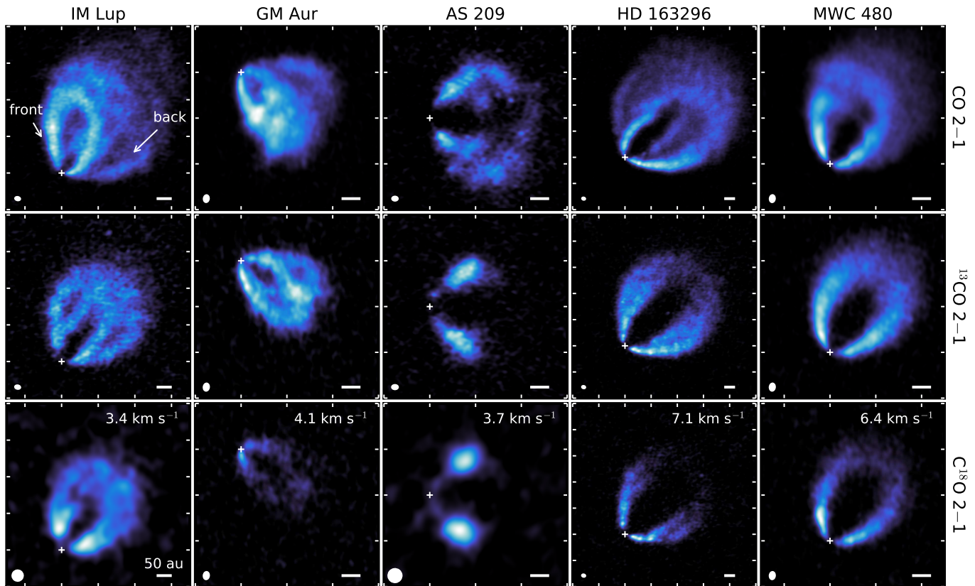
Figure 1. Representative channels for the MAPS sample, ordered from left to right by increasing stellar mass (see Table 1 in Oberg et al. (2021)), for CO 2–1, ^{13}\text{CO} 2–1, and \text{C}^{18}\text{O} 2–1. Both sides of the disk are visible and can be used to fit for the emitting layer. The \text{C}^{18}\text{O} 2–1 images in IM Lup and GM Aur have been tapered to 0''.30 , as described in Section 4.1. LSRK velocities are shown in the upper right corner and the plus symbol indicates the disk center. Axes are angular offsets from the disk center with 1'' tick marks. An arcsinh color stretch has been applied to highlight faint outer structures.
