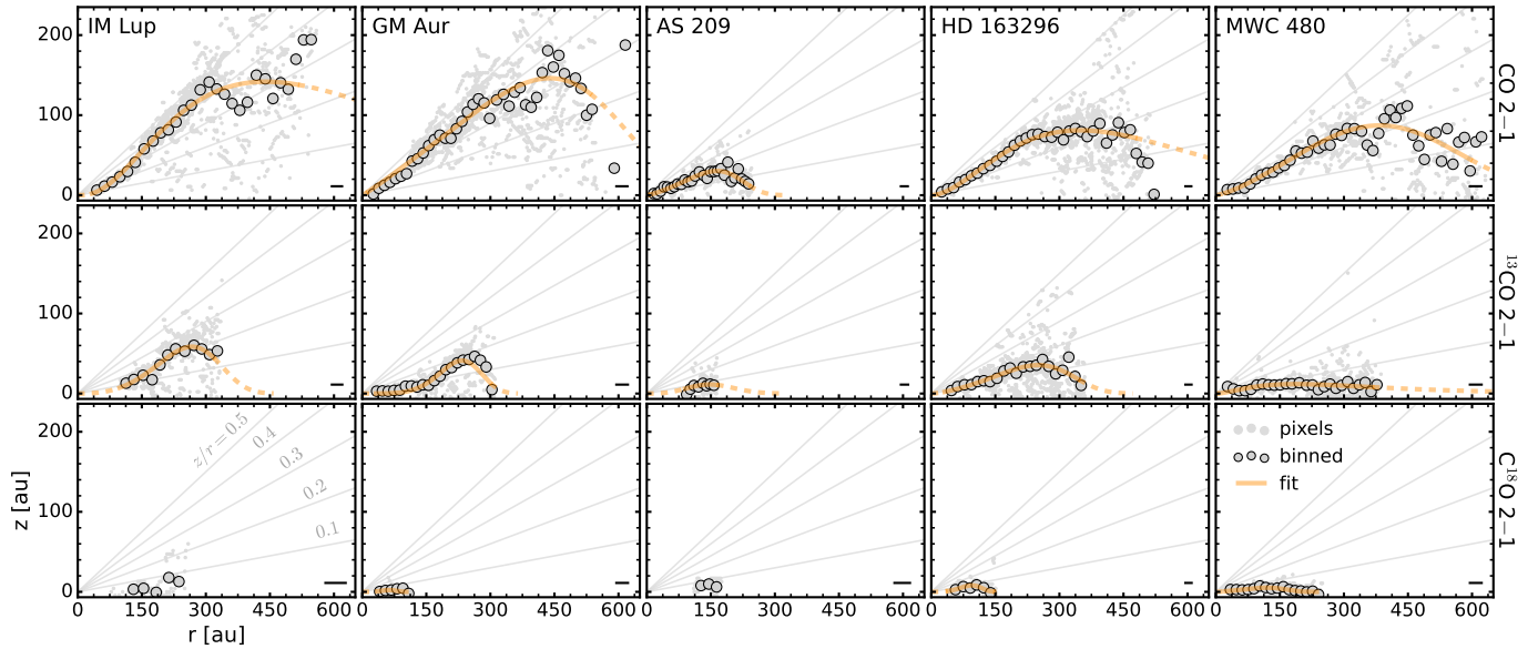
Figure 4. Emission surfaces for CO 2–1, ^{13}\text{CO} 2–1, and \text{C}^{18}\text{O} 2–1 in all MAPS sources. Large gray points show radially-binned surfaces and small, light gray points represent individual measurements. The orange lines show the exponentially-tapered power law fits from Table 1. The solid lines show the radial range used in the fitting, while the dashed lines are extrapolations. The \text{C}^{18}\text{O} 2–1 surfaces in IM Lup and AS 209 are tentative and were derived from the tapered ( 0''.30 ) images. Lines of constant z/r are shown in gray. The FWHM of the major axis of the synthesized beam is shown in the bottom right corner of each panel.
