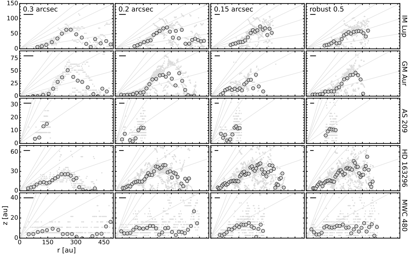
Figure 19. ^{13}\text{CO} 2–1 emission surfaces derived using different spatial resolutions. Otherwise, as in Figure 18.
