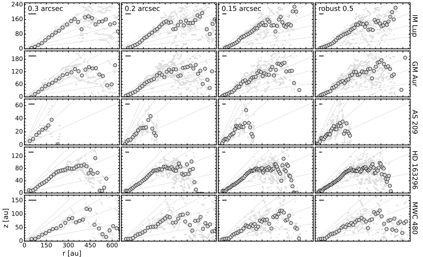
Figure 18. ^{12}\text{CO} 2–1 emission surfaces derived using images with different angular resolutions (see Table 5 in Oberg et al. 2021). Large, gray points show a consistent radial binning of 1/2\times the beam major axis of each image, while small, light gray points represent individual measurements. Lines of constant z/r from 0.1 to 0.5 in increments of 0.1 are shown in gray. The FWHM of the major axis of the synthesized beam is shown in the upper left corner of each panel.
