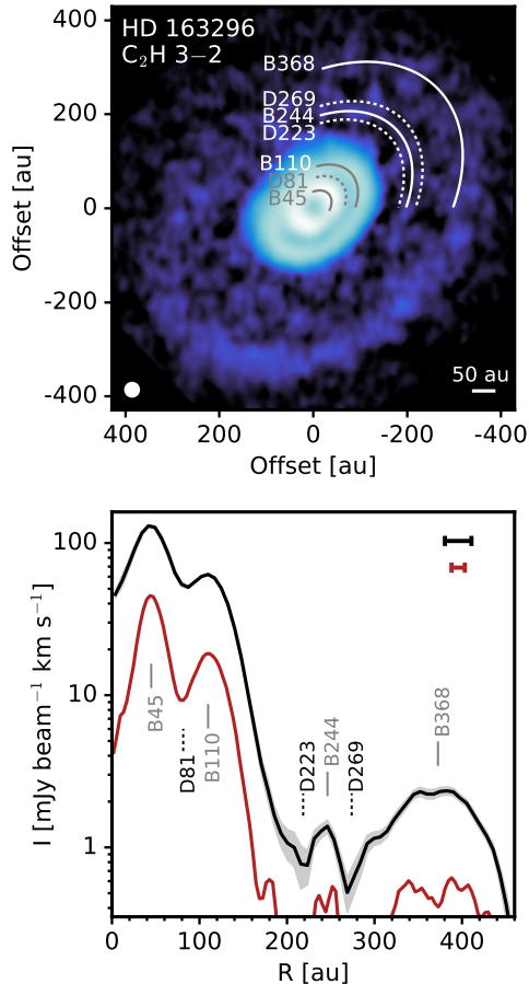
Figure 13. Zeroth moment map (top) and radial intensity profile (bottom) of C_2H 3-2 in HD 163296. An arcsinh color stretch has been applied to the zeroth moment map. The red and black curves show the 0''.15 and 0''.30 resolution profiles, respectively.
