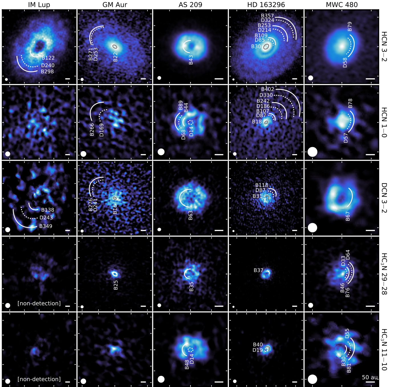
Figure 6. Zeroth moment maps of HCN, DCN, and HC 3 N lines for the MAPS sample, ordered from left to right by increasing stellar mass (see Table 1 in Oberg et al. (2021)). Axes are angular offsets from the disk center with each white tick mark represents a spacing of 1''. Color stretches were individually optimized and applied to each panel to increase the visibility of substructures. Care should thus be taken when comparing between panels, and instead, we recommend using the corresponding radial profiles in Figure 12 for this purpose. Chemical substructures from Table 3 in the form of rings and gaps are marked by solid and dotted arcs, respectively, with azimuthal extents and colors chosen for maximal visual clarity. The synthesized beam and a scale bar indicating 50 au is shown in the lower left and right corner, respectively, of each panel.
