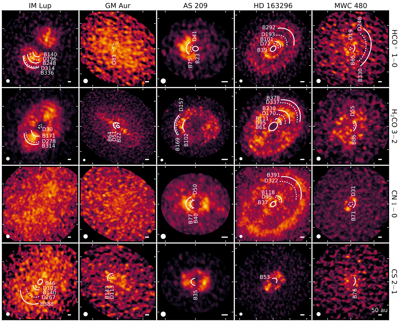
Figure 28.3. Peak intensity maps of \text{HCO}^+ , \text{H}_2\text{CO} , \text{CN} , and \text{CS} lines. Otherwise, as in Figure 3.
