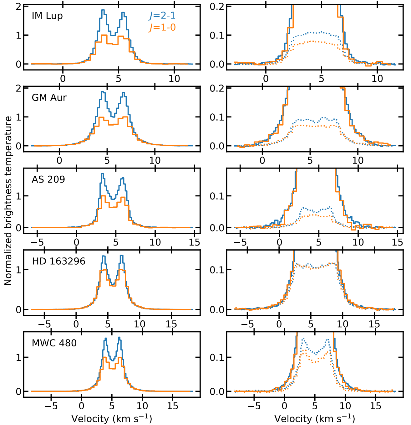
Figure 8. Comparison of the ^{13}\text{CO} J=2-1 (blue) and ^{13}\text{CO} J=1-0 (orange) line profiles. The profiles are normalized to the J=1-0 line. The left figure shows the full line profile, while the right shows a more constrained brightness temperature range, with spectra extracted with a 1'' aperture as dotted lines. The profiles are scaled to a brightness temperature scale assuming Rayleigh–Jeans law, which underestimates the J=2-1 line strength (see Sec. A.2). For velocities close to the systemic value, the J=2-1 line is consistently brighter than the J=1-0 line, indicating that the ^{13}\text{CO} flux is either optically thin, or that the J=2-1 flux comes from a warmer layer than the J=1-0 . In the line wings however, it seems that both lines are equally bright. This indicates that both the J=2-1 and the J=1-0 lines are optically thick.
