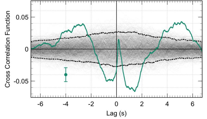
Figure A1. The g_s band vs X-ray CCF from epoch 4, averaged over 162 segments 10s in size, is shown in green – similar to that seen in Figure 3, but without binning. A representative error bar is plotted. The faded grey area is 1000 overlapping simulated correlation functions, and the black dotted lines are the 5% and 95% intervals of all the simulations. The feature at -3s, noted in Section 4.4, is above this significance line. The -1s feature in epoch 6 was similarly found to be significant.
