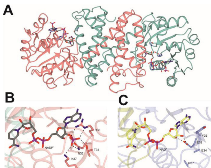
Figure 1. Structures of ( R )-IRED- M s wild-type and NADH-IRED- M s. A: Dimeric structure of ( R )-IRED- M s in complex with NADP + ; B: NADP + binding in ( R )-IRED- M s; C: NAD + binding in NADH-IRED- M s. Selected interactions between the cofactors and the active-site side-chains are indicated by black dashed lines. The side chains of E34 and R37 are absent in C as they could not be modelled.
