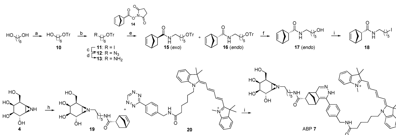
Scheme 1. Synthesis of ABP 7 . Reagents and conditions: a) TrCl, pyridine, CH_2Cl_2 , rt, 90 min, 95%; b) imidazole, PPh_3 , I_2 , Et_2O , CH_3CN , rt, overnight, 80%; c) NaN_3 , DMF, 80 °C, overnight, quant; d) polymer-bound PPh_3 , H_2O , THF, 48 h, quant; e) norbornene-OSu, DIPEA, DCE, rt, overnight, 15 : 28%, 16 : 68%; f) p -toluenesulfonic acid, CH_2Cl_2 , MeOH, rt, overnight, 86%; g) PPh_3 , I_2 , imidazole, THF, reflux, 1.5 h, 73%; h) 18 , K_2CO_3 , DMF, 75 °C, overnight, 12%; i) Cy5 tetrazine 20 , MeOH, overnight, 87%.
