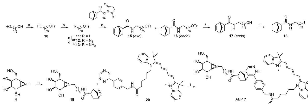
Scheme 1. Synthesis of ABP 7 . Reagents and conditions: a) TrCl, pyridine, CH 2 Cl 2 , rt, 90 min, 95%; b) imidazole, PPh 3 , I 2 , Et 2 O, CH 3 CN, rt, overnight, 80%; c) NaN 3 , DMF, 80 °C, overnight, quant; d) polymer-bound PPh 3 , H 2 O, THF, 48 h, quant; e) norbornene-OSu, DIPEA, DCE, rt, overnight, 15 : 28%, 16 : 68%; f) p -toluenesulfonic acid, CH 2 Cl 2 , MeOH, rt, overnight, 86%; g) PPh 3 , I 2 , imidazole, THF, reflux, 1.5 h, 73%; h) 18 , K 2 CO 3 , DMF, 75 °C, overnight, 12%; i) Cy5 tetrazine 20 , MeOH, overnight, 87%.
