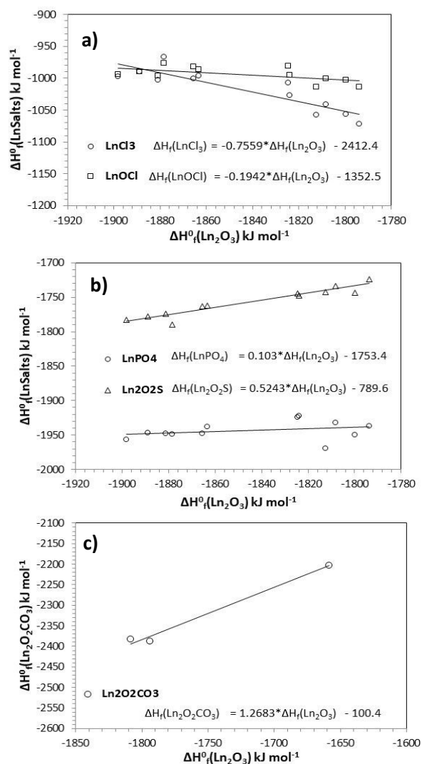
Figure 1. Relationship between \Delta H_f^\circ(\text{Ln}_2\text{O}_3) and \Delta H_f^\circ(\text{LnSalt}) for a) \text{LnCl}_3 and \text{LnOCl} , b) \text{LnPO}_4 and \text{Ln}_2\text{O}_2\text{S} and c) \text{Ln}_2\text{O}_2\text{CO}_3 . Pm, Eu and Yb were excluded from all analysis and for \text{Ln}_2\text{O}_2\text{CO}_3 only La, Nd and Eu were considered.
