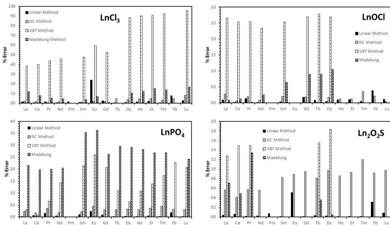
Figure 2 Comparison between estimated and experimental values of the enthalpy of formation for \text{LnCl}_3 , \text{LnOCl} , \text{LnPO}_4 and \text{Ln}_2\text{O}_2\text{S}
