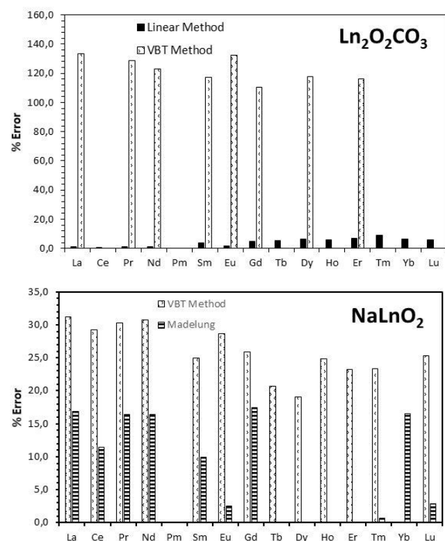
Figure 3 Comparison between estimated values of the enthalpy of formation with the group contribution, VBT and Madelung methods for \text{Ln}_2\text{O}_2\text{CO}_3 and \text{NaLnO}_2
