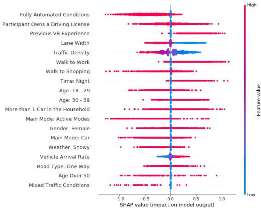
Figure 6: Plot summary of the effects of all the covariates based on the SHAP Values
