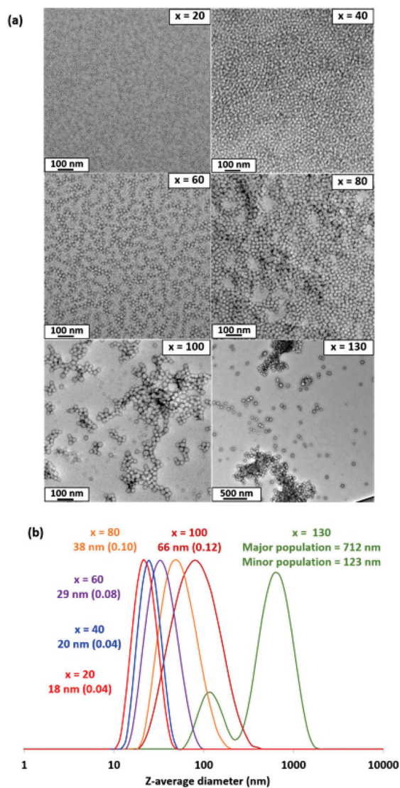
Fig. 2 (a) Representative TEM images and (b) DLS particle size distributions obtained for a series of PGMA 50 -PMMA x nanoparticles prepared by RAFT aqueous emulsion polymerization of MMA where the target PMMA DP ( x ) is 20, 40, 60, 80, 100 or 130. DLS indicates a bimodal particle size distribution in the latter case owing to nanoparticle flocculation.
