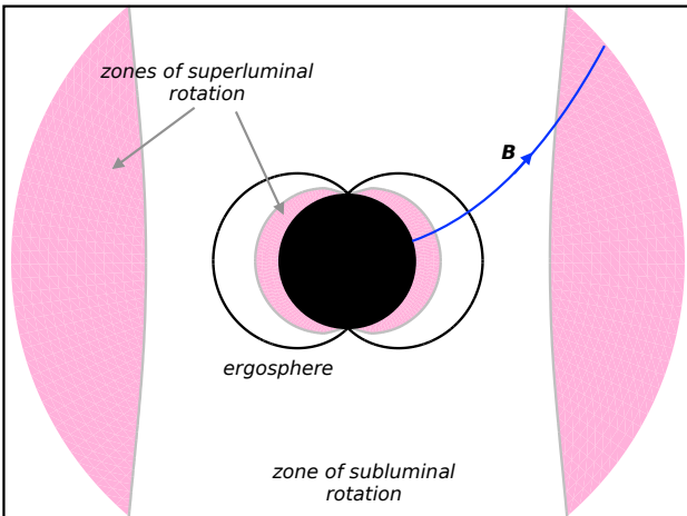
Figure 4. Superluminal and subluminal zones for rotation with \Omega = 0.5\Omega_h , where \Omega_h = a/(r_+^2 + a^2) is the angular velocity of the black hole with a = 1 .
