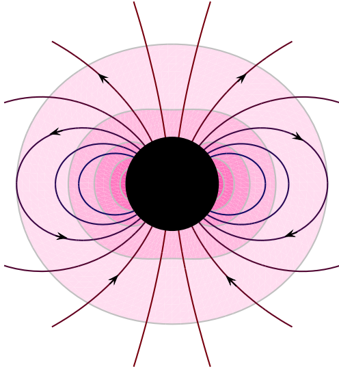
Figure 5. Magnetic field lines and electrostatic potential of Wald's solution for an electrically-charged BH with a = 1 and B_0 = 0 . Contours of (2/q)\Phi are 0.6, 0.9, 1.2, 1.5 and 1.8 in the order of decreasing intensity of colour/shade. The magnetic field lines correspond to (2/q)A_\phi = 0.02, 0.2, 0.4, 0.6, 0.8 , and 1.0
