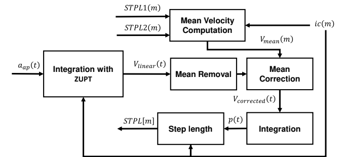
Fig. 3 Block diagram of STPL7. After the integration of a_{ap}(t) with zero-velocity update assumption, mean value of V_{linear}(t) at each gait cycle was replaced with a new mean, V_{mean}(m) , computed according to (16) to obtain V_{corrected}(t) . Then, resulted signal was integrated and (17) was used to compute step length.
