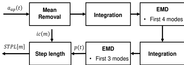
Fig. 2 Block diagram of STPL6. After removing mean of a_{ap}(t) and integrating the zero-mean signal, EMD was used to keep the first 4 intrinsic modes. Then, another integration and EMD were applied on the resulted signal to generate p(t) by the first 3 intrinsic modes. Then, (14) was used to compute step length.
