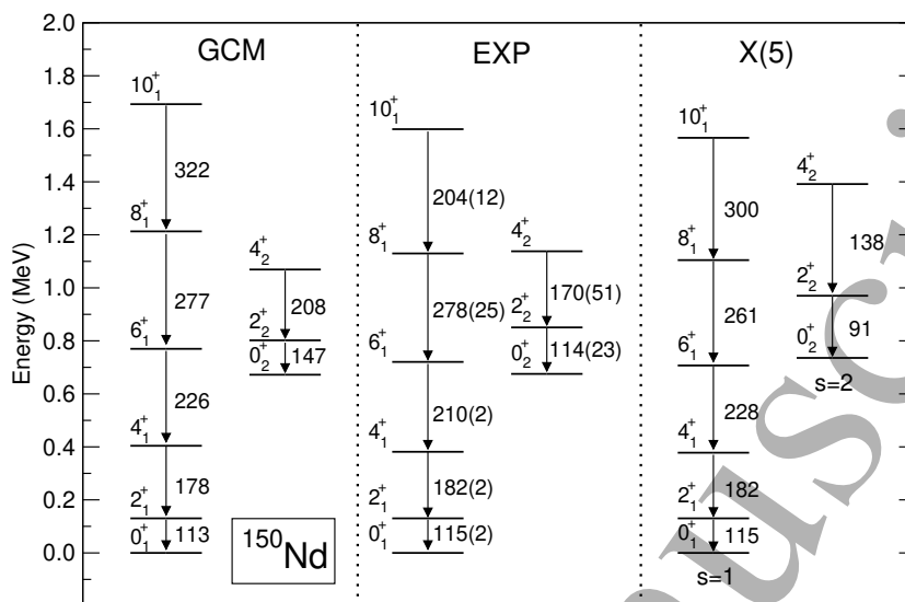
Figure 16. The particle-number-projected generator-coordinate-method spectrum of ^{150}\text{Nd} (left), compared with experiment (middle), and the X(5) -symmetry predictions (right). Figure reprinted with permission from Nikšić et al. (2007). Copyrighted by the American Physical Society.
