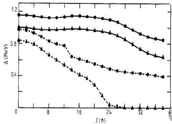
Figure 8. Pairing correlations in ^{168}\text{Hf} as a function of angular momentum. Gap parameters for protons (circles) and neutrons (triangles) obtained by a variation after number projection (full curves) and by pure mean-field theory (dashed curves). Republished with permission of Institute of Physics, from Mutz and Ring (1984) ; permission conveyed through Copyright Clearance Center, Inc.
