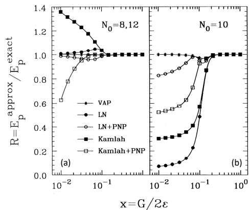
Figure 6. Pairing energies in the two-level model obtained in Zheng et al. (1992) within the variation after projection (VAP) (asterisks), Kamlah (full squares), and Lipkin-Nogami (full circles) approximations, relative to the exact values and plotted for N_0 = \Omega = 10 (right), and N_0 = \Omega \pm 2 (left). The energies resulting from the exact particle-number projection of Kamlah (open squares) and Lipkin-Nogami (open circles) states are shown for comparison. The critical value of x is x_c = 1/9 . Figure reprinted with permission from Dobaczewski and Nazarewicz (1993) . Copyrighted by the American Physical Society.
