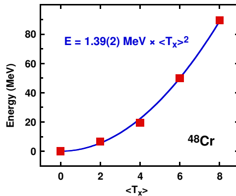
Figure 5. Excitation energies of ^{48}\text{Cr} isocranked to \langle T_x \rangle = 0, 2, 4, 6, \text{ and } 8 (squares) (Sato et al., 2013). The solid line represents the parabolic fit.
