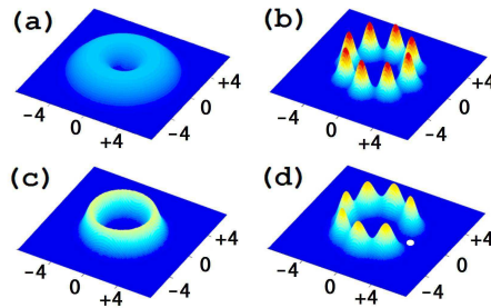
Figure 23. Single-particle densities and conditional probability distributions for N = 8 bosons in a rotating toroidal trap, see Romanovsky et al. (2006) for details. (a) Gross-Pitaevskii single-particle density. (b) UBHF single-particle density exhibiting breaking of the circular symmetry. (c) Rotating-boson-molecule single-particle density exhibiting circular symmetry. (d) Conditional probability distribution for the rotating-boson-molecule wave function (PRJ wave function, symmetry restored) revealing the hidden point-group symmetry in the intrinsic frame of reference. The fixed (observation) point is denoted by a white dot. The rotating-boson-molecule ground-state angular momentum is L = 16 . Figure reprinted with permission from Romanovsky et al. (2006) . Copyrighted by the American Physical Society.
