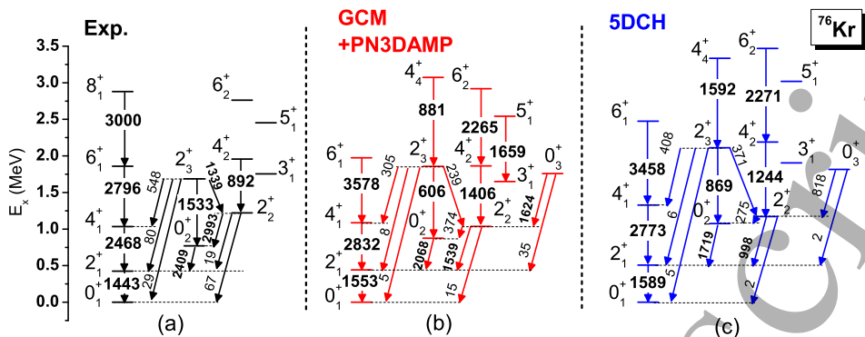
Figure 18. Low-lying spectra and B(E2) values (in e^2 \text{fm}^4 ) of ^{76}\text{Kr} . Experimental data (a) are compared with the full relativistic generator-coordinate-method calculations with particle-number and three-dimensional angular-momentum-projection (b) and with five-dimensional Bohr Hamiltonian results (c). Figure reprinted with permission from Yao et al. (2014). Copyrighted by the American Physical Society.
