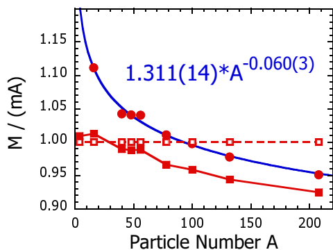
Figure 7. Exact masses ( M = mA , open squares) and the Peierls-Yoccoz masses M = \mathcal{M}_{\text{PY}} , equation (149), calculated in doubly magic nuclei before (full circles) and after (full squares) including the Lipkin operator. Republished with permission of Institute of Physics, from Dobaczewski (2009); permission conveyed through Copyright Clearance Center, Inc.
