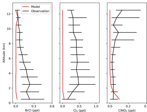
Figure 10. (a) Vertical profiles of BrCl, Cl 2 , and CINO 2 mixing ratios from the ATom-3 campaign over the Pacific and Atlantic in September–October 2017. Observations are medians and 25th–75th percentiles in 1 km vertical bins. Model values are medians sampled along the flight tracks. (b) Same as Fig. 10a but for the ATom-4 campaign in April–May 2018.
