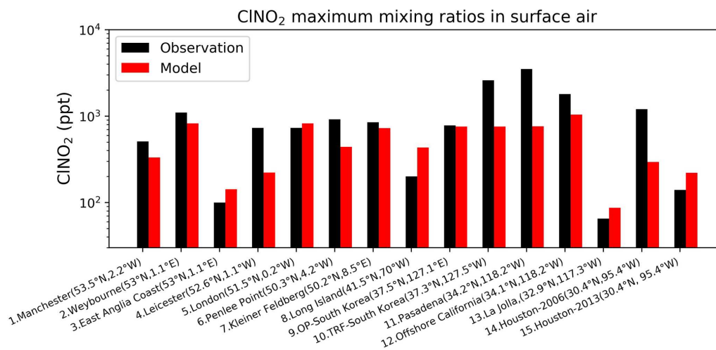
Figure 8. Surface air mixing ratios of ClNO 2 at coastal and island sites, arranged from left to right in order of decreasing latitude. Observed (black) and modeled (red) values are maxima for the reporting period. Model maxima are based on hourly values sampled at the same location and time period as the observations. References: (1) Priestley et al. (2018), (2, 4, 6) Sommariva et al. (2018), (3, 5) Bannan et al. (2017), (7) Phillips et al. (2012), (8) Kercher et al. (2009), (9, 10) Jeong et al. (2018), (11) Mielke et al. (2013), (12) Riedel et al. (2013), (13) Kim et al. (2014), (14) Osthoff et al. (2008), (15) Faxon et al. (2015).
