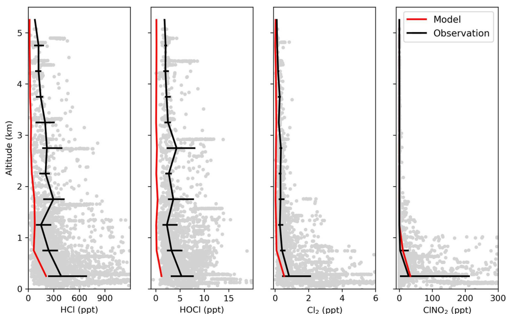
Figure 9. Vertical profiles of HCl, HOCl, Cl 2 and nighttime CINO 2 mixing ratios during the WINTER campaign over the eastern US and offshore in February–March 2015. Observations are shown as individual 1 min data points, with medians and 25th–75th percentiles in 500 m vertical bins. CINO 2 data exclude during the daytime (10:00–16:00LT), when mixing ratios are near zero in both the observations and the model. Model values are shown as medians sampled along the flight tracks.
