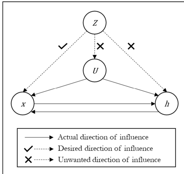
Fig 1. Directed Acyclic Graph (DAG) depicting the role of an instrumental variable ( Z ) in estimating the causal relationship between health spending ( X ) and health outcomes ( h ) with unobserved covariates ( U )
