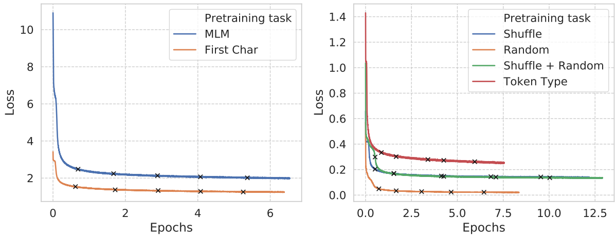
Figure 5: The loss curves for BERT-SMALL models. Each × denotes a checkpoint pretrained for 1 \leq n \leq 5 day(s).
