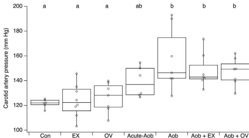
Figure 1. Hypertension after chronic abdominal aortic stenosis
