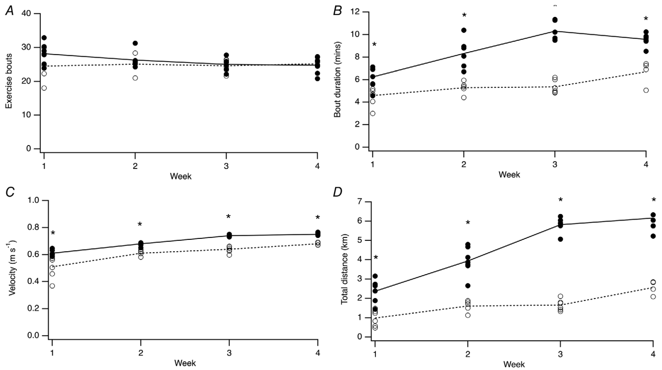
Figure 2. Impaired voluntary wheel-running exercise performance after abdominal aortic banding While inclination to exercise was undiminished (A), bout duration (B), velocity (C) and total distance travelled (D) were reduced in banded animals (Aob+EX: dashed line) compared with exercise controls (EX: continuous line). Interpolation lines fitted through the mean at each timepoint for each group. Asterisks denote statistical significance between EX (N = 8) and Aob+EX (N = 7) at each timepoint (P < 0.05).
