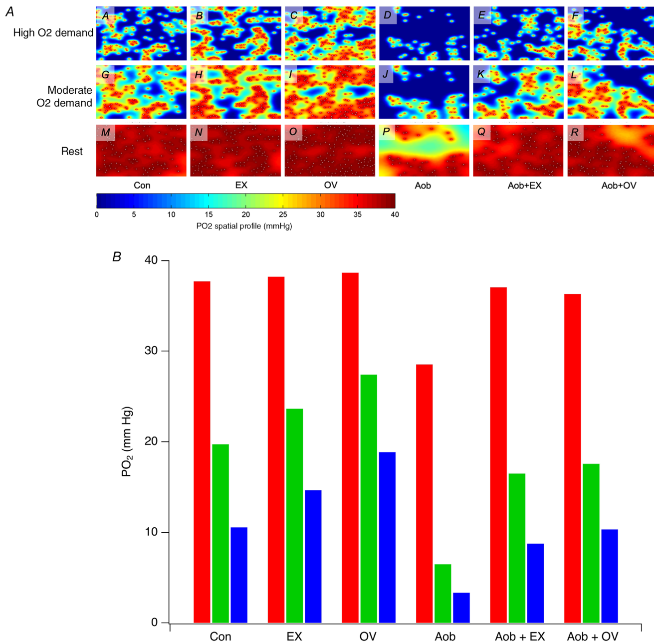
Figure 6. Simulation of muscle PO_2 at rest, moderate and high rates of oxygen consumption
