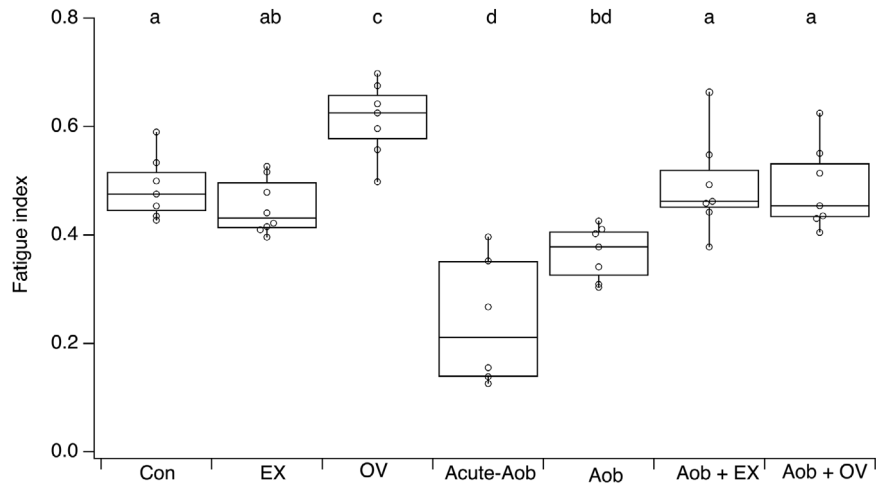
Figure 3. Impaired muscle fatigue resistance accompanied compensatory cardiac hypertrophy but recovered after intervention Fatigue index (FI) was reduced immediately after band application and remained impaired for 4 weeks without intervention (Aob: P = 0.039). Exercise (Aob+EX) and overload (Aob+OV) recovered fatigue resistance to control levels (both P = 0.999) despite the chronic effects of aortic banding. Group sizes were the same as in Fig. 1. Statistically significant differences between groups are denoted by letters; groups sharing the same letter were not different, those sharing none were statistically different (P < 0.05) as determined by ANOVA with Tukey's post hoc tests.
