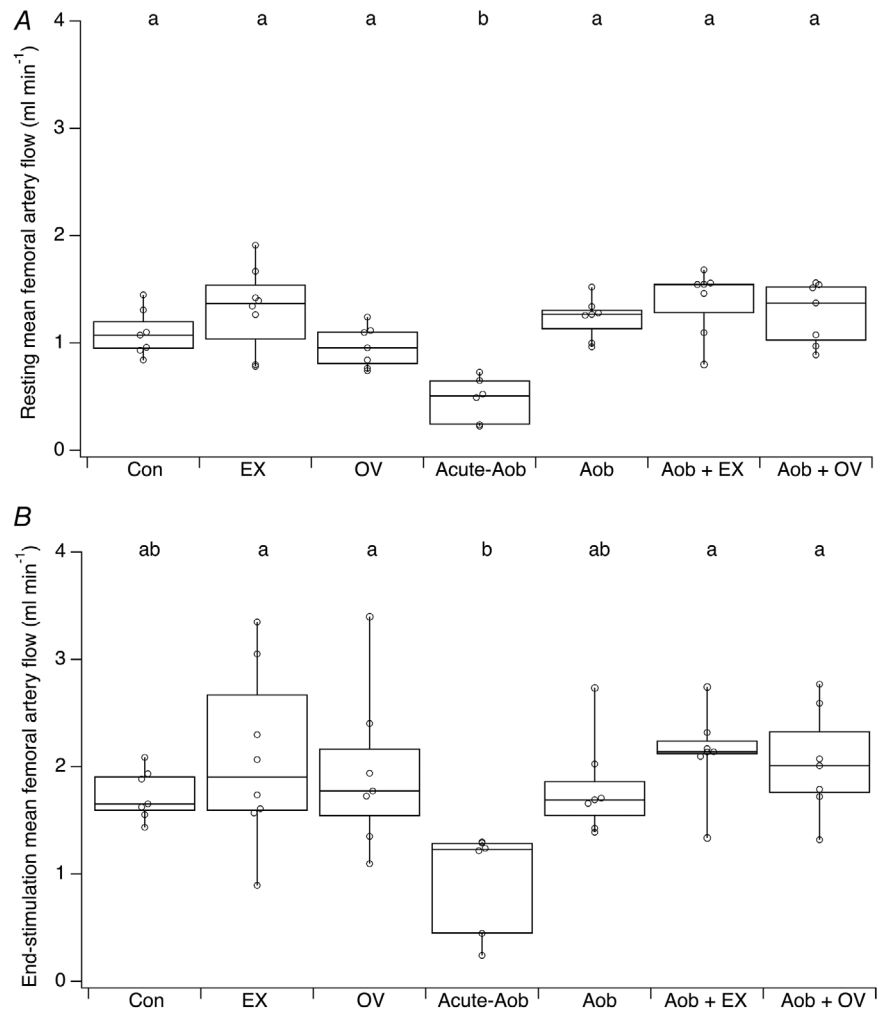
Figure 4. Resting (A) and end-stimulation (B) mean femoral artery blood flow A pronounced reduction in femoral blood flow occurred immediately after aortic stenosis (Acute-Aob) but was restored in chronically banded animals. Group sizes were the same as in Fig. 1. Statistically significant differences between groups are denoted by letters; groups sharing the same letter were not different, those sharing none were statistically different ( P < 0.05 ) as determined by ANOVA with Tukey's post hoc tests.
