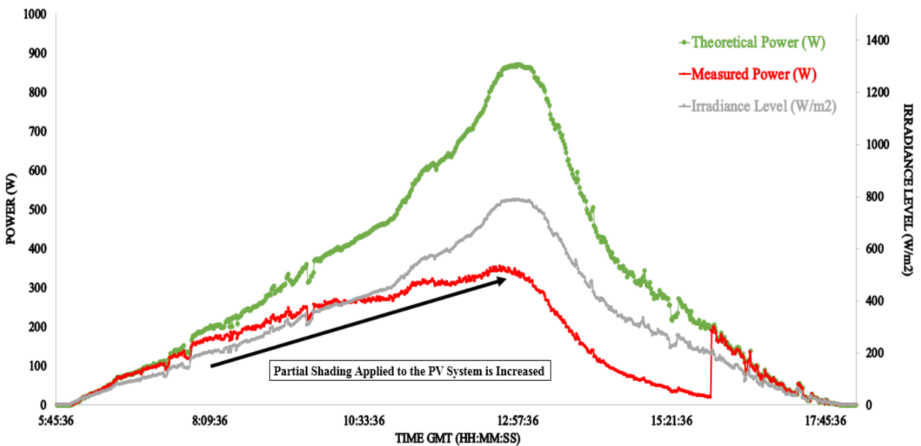
Fig. 6 Theoretical power vs. measured output power for a PS condition effects the examined PV system
