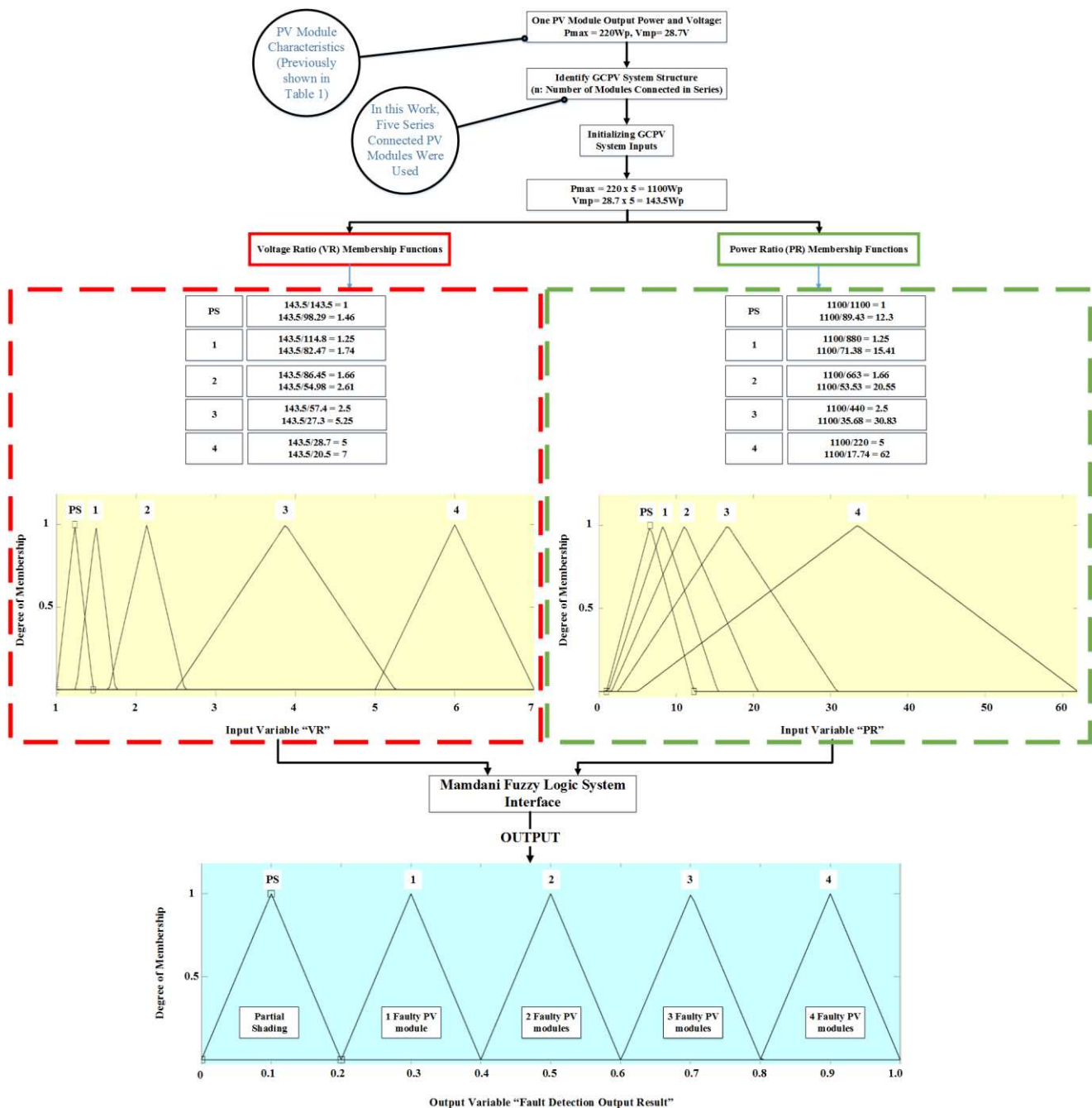
Fig. 3 Proposed fuzzy logic system interface
