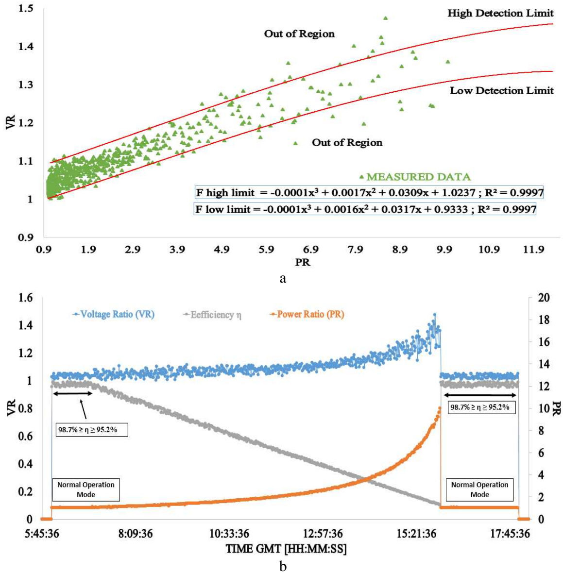
Fig. 7 Theoretical curves modelling vs. real time long term measured data a Theoretical detection limits for the PV system under PS conditions b Voltage power and efficiency variations for the tested experiment (PV system under PS conditions only)
