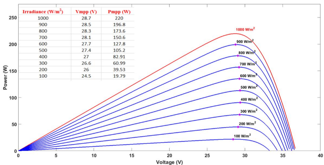
Fig. 1 P-V curve modelling under various irradiance levels and fixed PV module temperature (25 °C).
