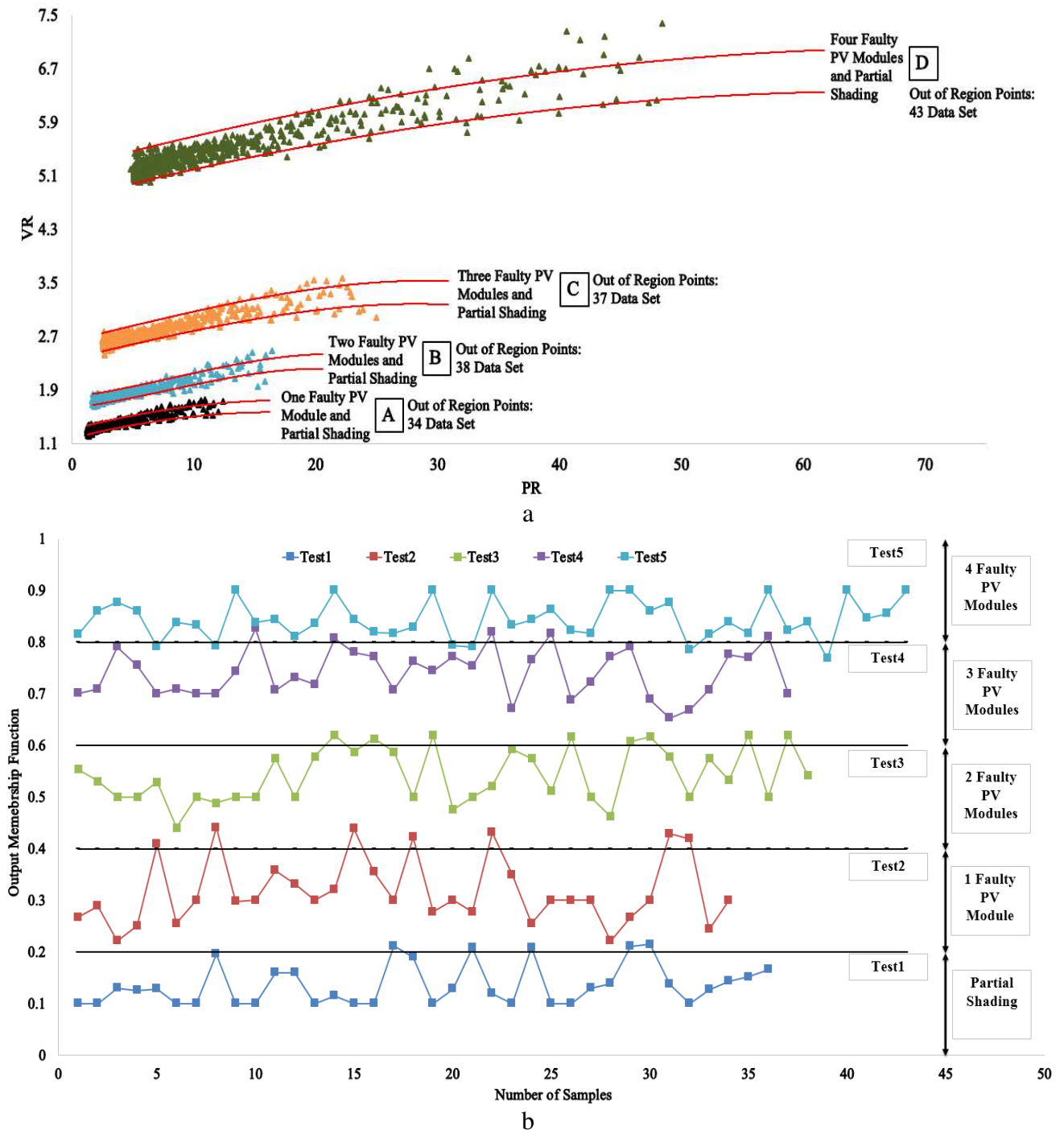
Fig. 8 Validate the proposed fuzzy logic system using various PV faulty conditions a Theoretical detection limits vs. real time long term data measurements b Out of region samples processed by the fuzzy logic system vs. the output membership function
