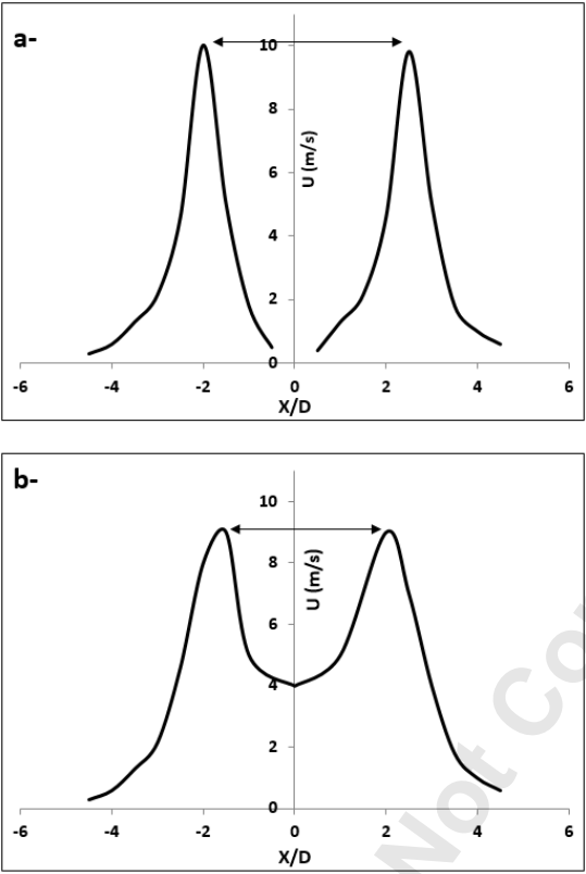
Figure 11: Radial velocity profile in the cross-stream direction ( X/D_o ) at location of Y/D_o = 3 for orifice spaced a) 10 mm and b) 5 mm ( f = 1000 Hz, V = 35 Vrms).
