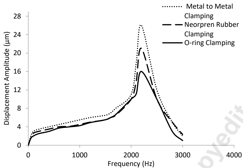
Figure 7: The diaphragm displacement amplitude at different excitation frequencies at constant excitation voltage of V_{rms} = 35 V.
