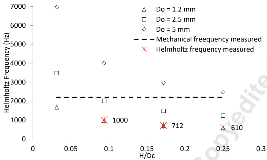
Figure 13: Calculated Helmholtz frequency against cavity height for three orifices diameters.
