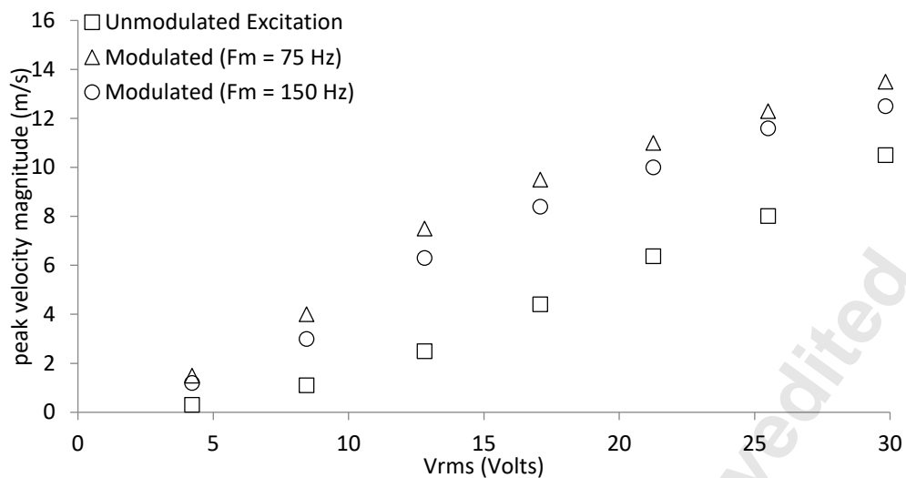
Figure 20: Peak jet velocity for both modulated and un-modulated wave at ( Y/D_o = 0.5, f_c = f_H = 1000 Hz).
