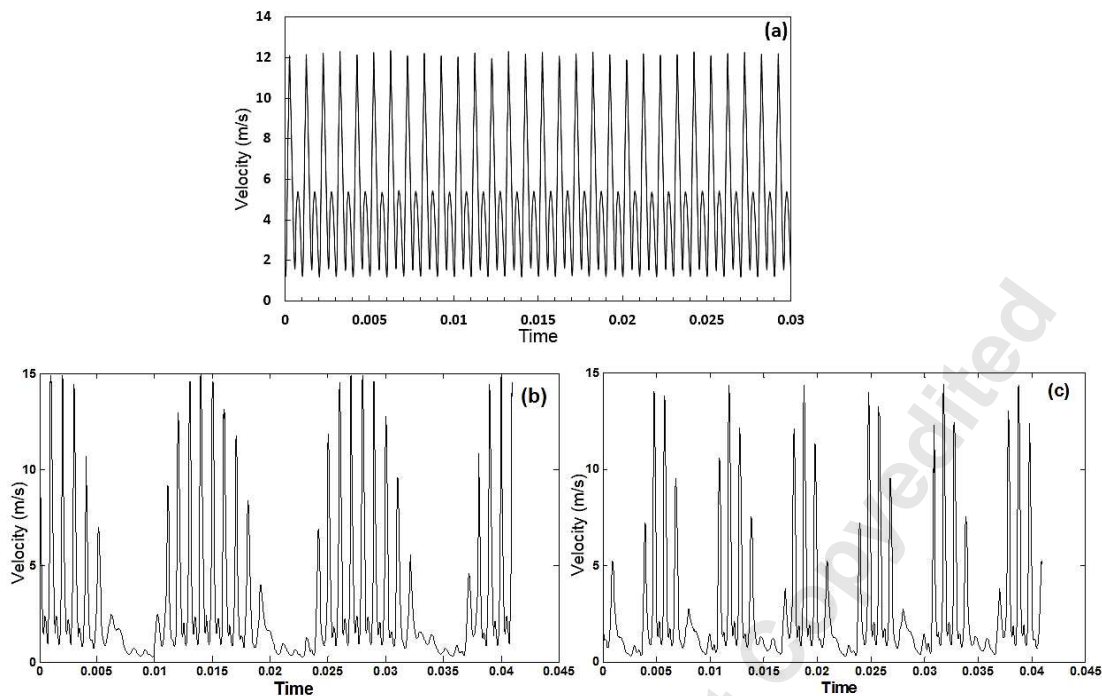
Figure 19: Synthetic jet velocity at V_{rms} = 35 volts for a) Un-modulated synthetic jets, b) Modulated wave ( f_c = 1000 Hz, f_m = 75 Hz), c) Modulated ( f_c = 1000 Hz, f_m = 150 Hz).
