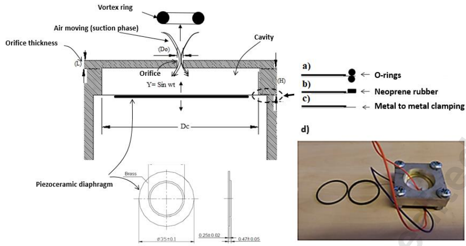
Figure 2: Different ways of clamping: a) between two O-rings; b) using a neoprene rubber on one side; c) metal to metal clamps; d) assembled actuator unit.
