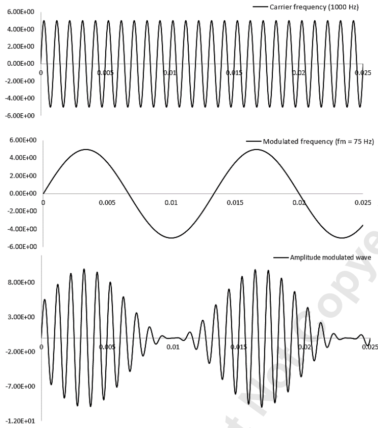
Figure 17: The creation of a modulated signal by adding a carrier with a modulated wave.
