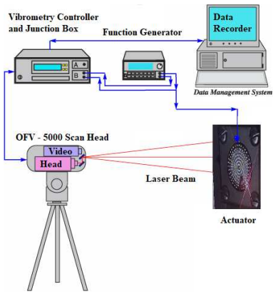
Figure 3: Polytec Scanning Vibrometer experimental setup.
