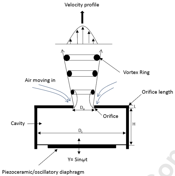
Figure 1: Schematic of SJA with piezo-ceramic diaphragm as active element.
