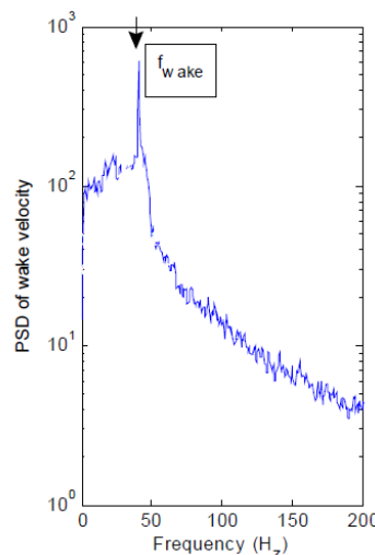
Figure 16: An example of PSD in a wake area airfoil trailing edge [37].
