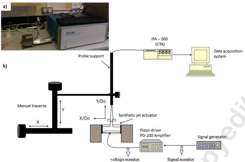
Figure 4: Photograph of experimental setup (a) and block diagram of instrument layout (b).
