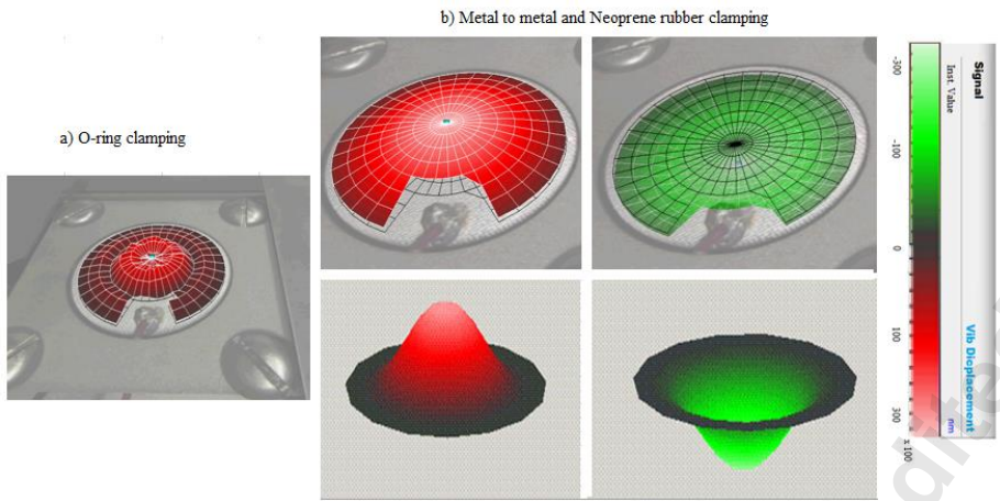
Figure 6: The clamping method effect on the actuator performance at different clamping methods a) O-ring clamping b) metal to metal and neoprene rubber clamping.
