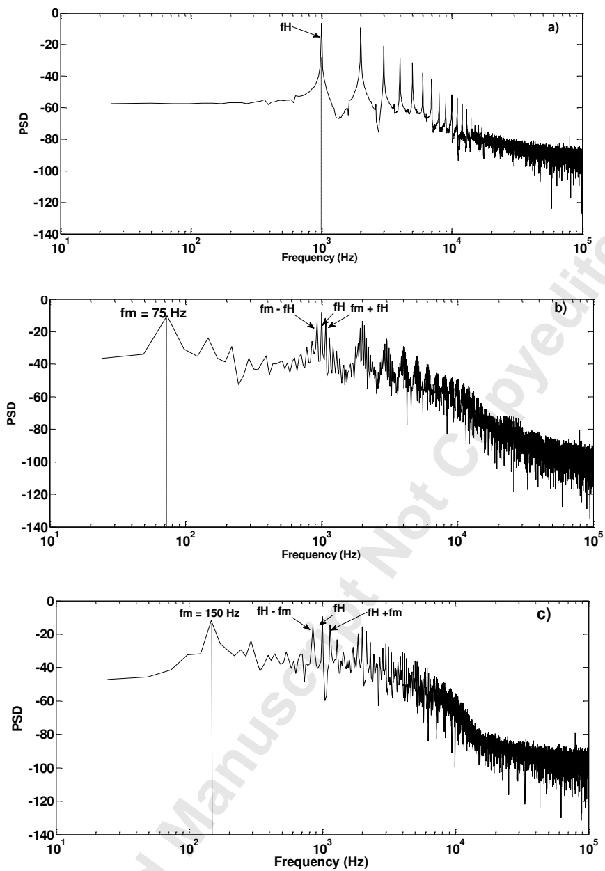
Figure 18: Power spectral density at Y/D_o = 0.5 , a) Un-modulated jets ( f_c = f_H = 1000 Hz), b) Modulated jets ( f_c = f_H = 1000 Hz, f_m = 75 Hz), c) Modulated jets ( f_c = f_H = 1000 Hz, f_m = 150 Hz).
