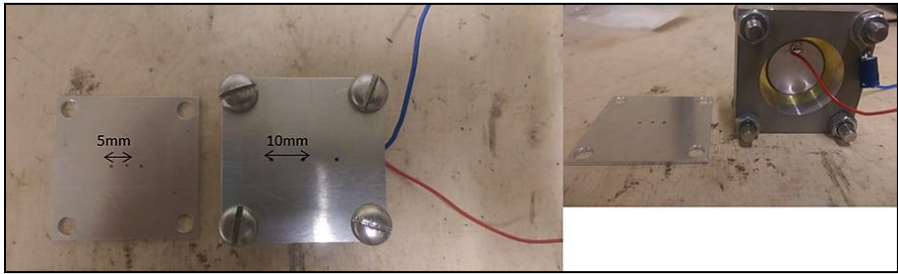
Figure 5: Experimental set-up of the most efficient orifice spacing study.
