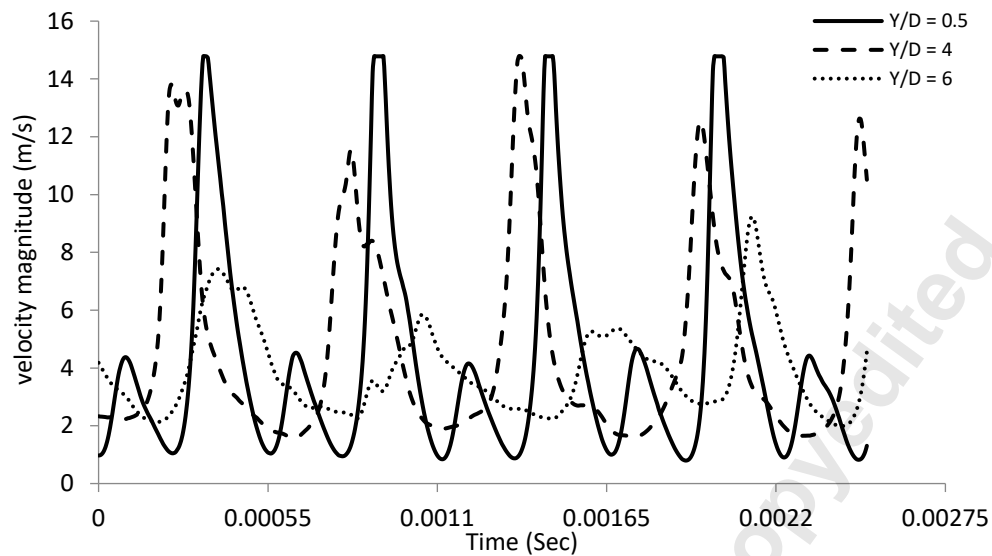
Figure 9: Time history of the velocity magnitude measured in the stream-wise at H/D_c = 0.093 ; Y/D_o = 0.5 ; Y/D_o = 4 and Y/D_o = 6 above the orifice centreline ( V_{rms} = 35 volt and excitation frequency = 1800 Hz).
