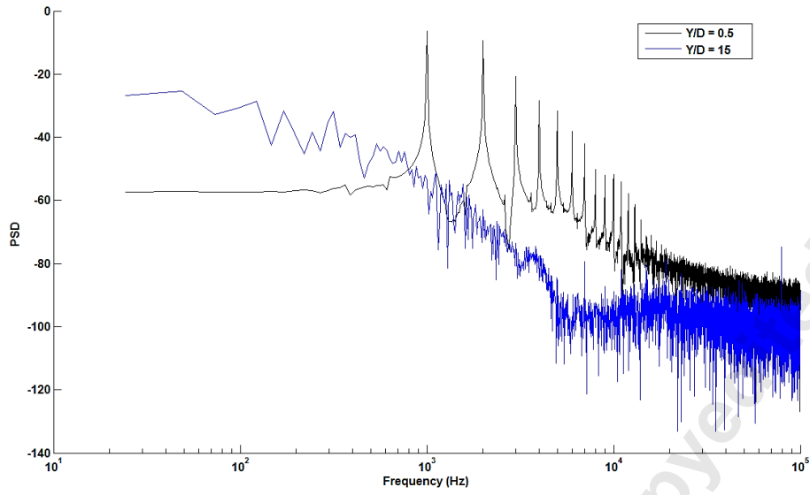
Figure 10: Power spectral density of z-plane velocity magnitude at H/D_c = 0.093 ; Y/D_o = 0.5 and Y/D_o = 15 above the orifice centreline ( V_{rms} = 35 volt and excitation frequency = 1800 Hz).
