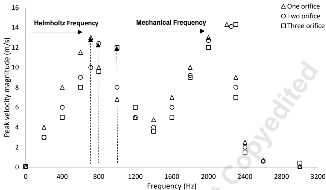
Figure 12: Experimental data of the frequency response of the synthetic jet actuator at different numbers of orifices ( V_{rms} = 35 volts, metal-to-metal clamping).
