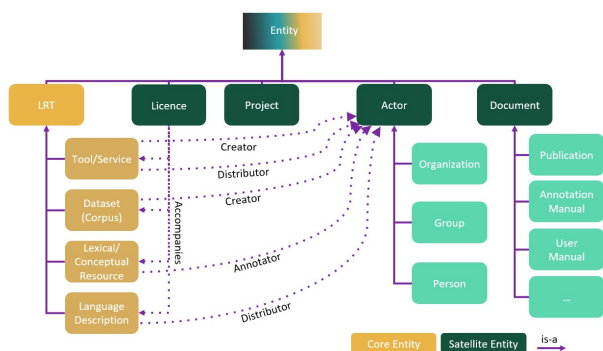
Figure 2: Entities covered by the ELG metadata schema
