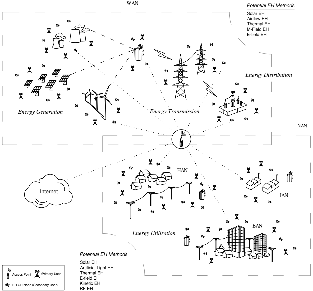
Fig. 3 Network Architecture of IoT-enabled SG.
